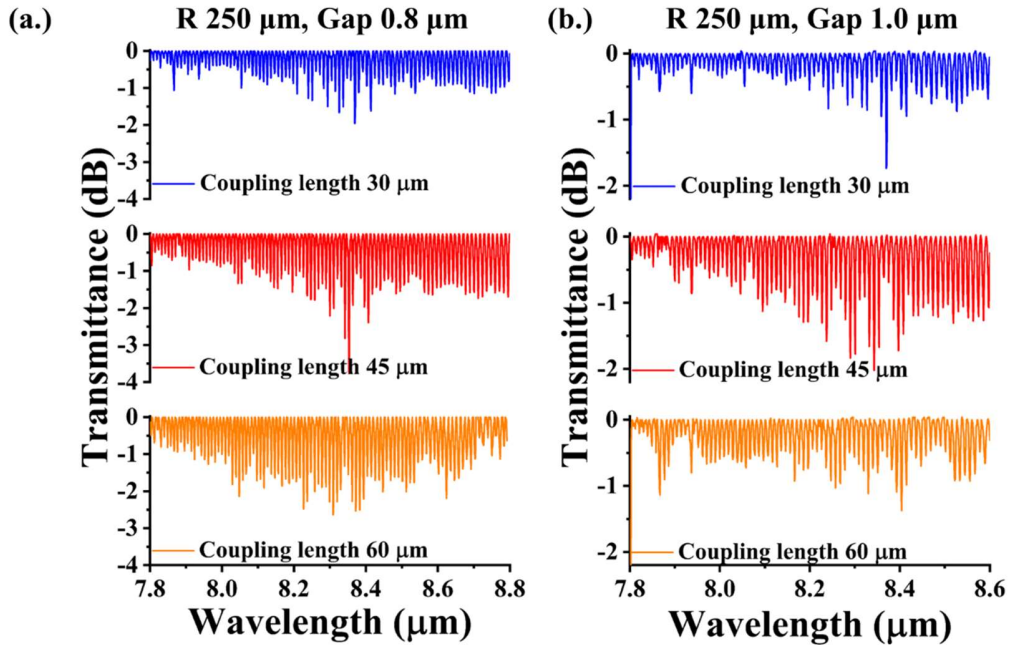
Fig.3. Experimental transmission spectra of the racetrack resonators in quasi TM-polarization with (a.) gap = 0.8 μm. (b.) gap = 1.0 μm, respectively, and for different lengths of the directional coupler (30, 45, and 60 μm). Broadband operation of the resonators is observed in all cases.
