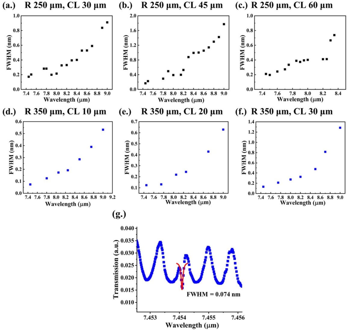
Fig.6. Resonance FWHM as a function of the wavelength for resonator with different radius and coupling lengths (the gap is fixed at 1 μm) : (a.) R = 250 μm, CL = 30 μm, (b.) R = 250 μm, CL = 45 μm, (c.) R = 250 μm, CL = 60 μm, (d.) R = 350 μm, CL = 10 μm, (e.) R = 350 μm, CL = 20 μm, and (f.) R = 350 μm, CL = 30 μm respectively. (g.) Example of resonator transmission as a function of the wavelength, at \lambda = 7.45 \mu\text{m} from the racetrack with the radius 350 μm and coupling length 10 μm, showing the highest Q-factor of 1.01 \times 10^5
