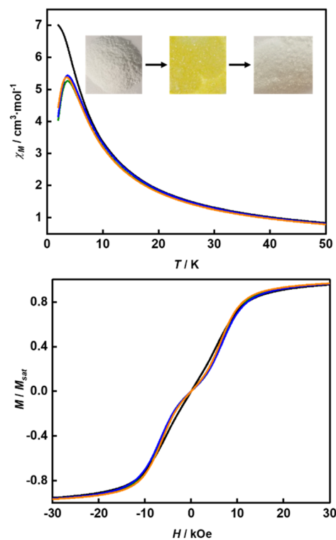
Fig. 6 Temperature-dependent \chi_M values (top) and M/M_{\text{sat}} vs. H plots at 1.9 \text{ K} (bottom) for 1 (green line), 1 –180 (black line), 1 –180– \text{CH}_3\text{OH} (blue line) and 1 –180– \text{H}_2\text{O} (orange line). Inset: the photos of powder samples of 1 (left), 1 –180 (middle) and 1 –180– \text{CH}_3\text{OH} (right).
