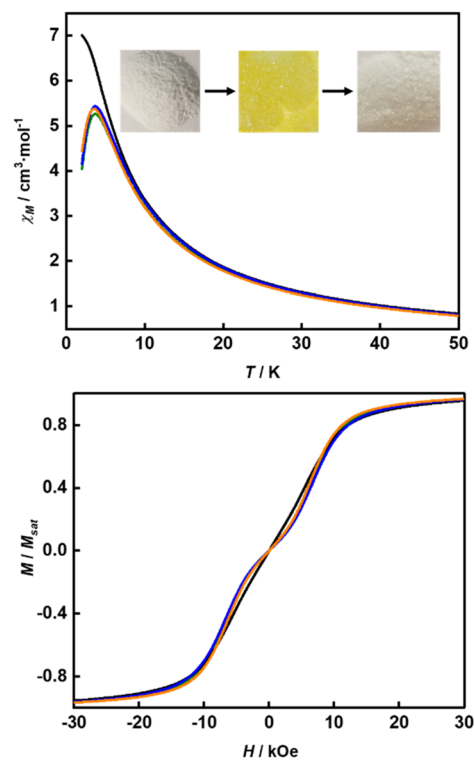
Fig. 6 Temperature-dependent \chi_M values (top) and M/M_{\text{sat}} vs. H plots at 1.9 K (bottom) for 1 (green line), 1–180 (black line), 1–180–CH 3 OH (blue line) and 1–180–H 2 O (orange line). Inset: the photos of powder samples of 1 (left), 1–180 (middle) and 1–180–CH 3 OH (right).
