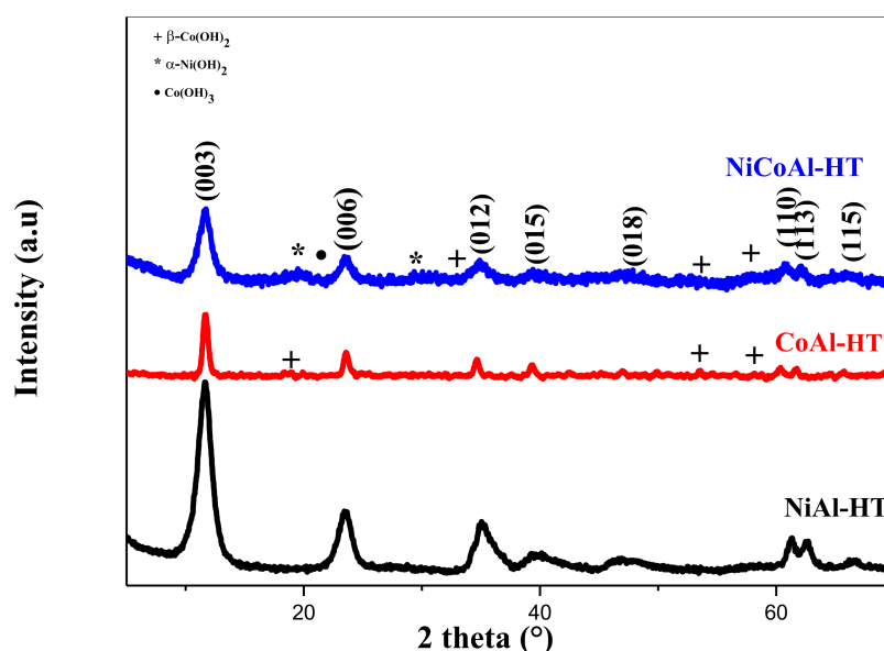
Figure 2. XRD patterns of: NiAl-HT, CoAl-HT, and NiCoAl-HT LDHs.
