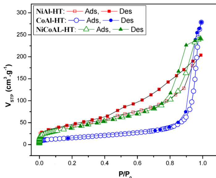
Figure 5. \text{N}_2 adsorption-desorption isotherms of: NiAl-HT, CoAl-HT, and NiCoAl-HT.
