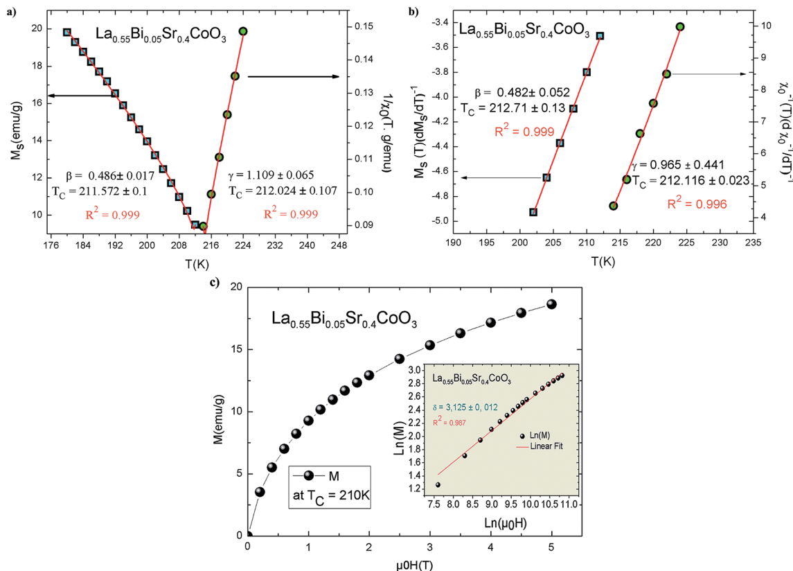
Fig. 6 (a) Spontaneous magnetization (left axis) and inverse initial susceptibility (right axis) vs. temperature for \text{La}_{0.55}\text{Bi}_{0.05}\text{Sr}_{0.4}\text{CoO}_3 . (b) K - F construction for determining the critical exponents and T_C ; solid lines are the fitted data. (c) Critical isotherm of M vs. \mu_0 H for \text{La}_{0.55}\text{Bi}_{0.05}\text{Sr}_{0.4}\text{CoO}_3 . Inset: \ln - \ln scale for M vs. \mu_0 H .
