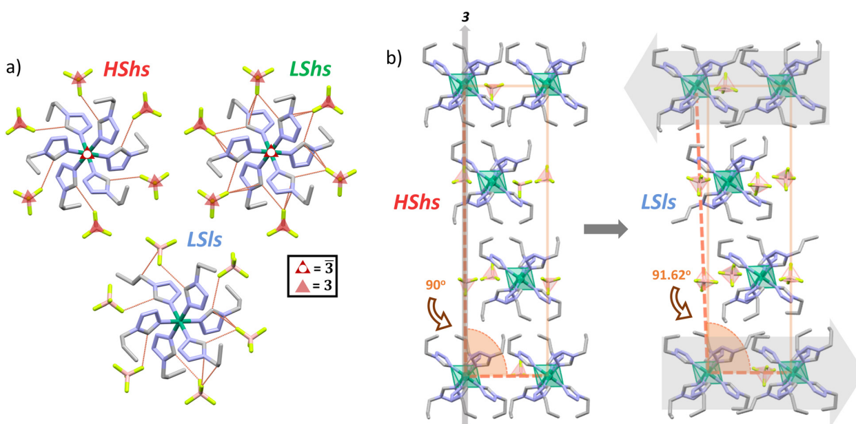
Fig. 6 a) Intermolecular contacts between the cationic complex located on \bar{3} symmetry and \text{BF}_4^- counter-anions located on 3-fold symmetry axis in the HShs and LShs. In the LSlS the inter-molecular contacts are no more symmetry-equivalent. b) Ferroelastic distortion upon the R\bar{3} \rightarrow P\bar{1} transformation of the lattice viewed along the b axis of the pseudo-rhombohedral lattice, with a shear strain shown by the grey arrows. Hydrogen atoms and possible disorder of both n -propyl groups and \text{BF}_4^- counter-anions are omitted for clarity.
