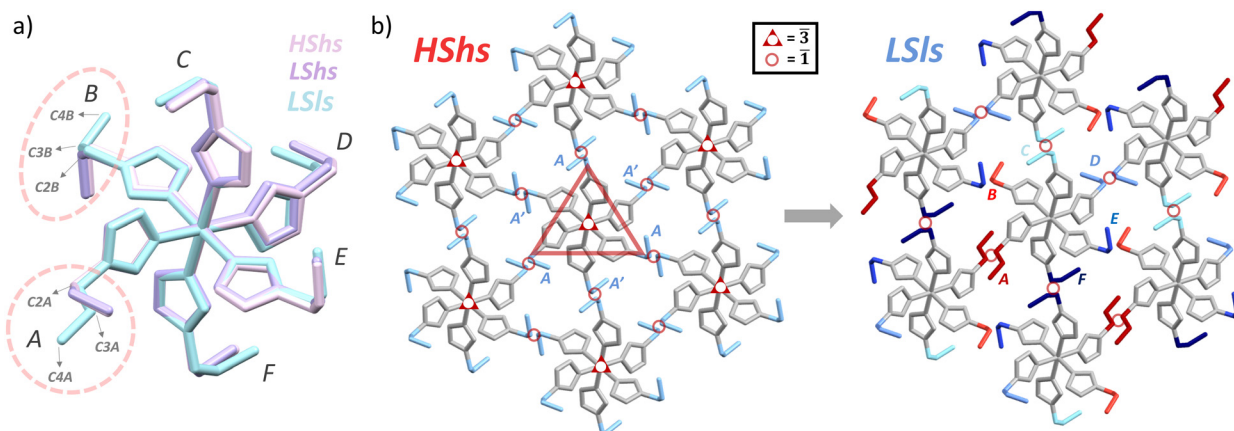
Fig. 5 a) Minimised overlay of the cationic complex in the HShs (pink), LShs (purple) and LSlS (green) phases showing the conformational changes of n -propyl groups (C2A–C3A–C4A and C2B–C3B–C4B) in circled areas. Disorder of n -propyl group in the HShs phase is omitted for clarity. b) Symmetry-breaking associated with rearrangement of propyl groups, viewed along the c axis of the (pseudo) rhombohedral lattice. In the HShs and LShs states, the cations are located on \bar{3} symmetry with equivalent A–B–C–D–E–F n -propyl groups. The cations are related by 3-fold and inversion symmetry. In the LSlS phase the 3-fold axis is lost and some \bar{1} symmetry elements are kept in the P\bar{1} lattice.
