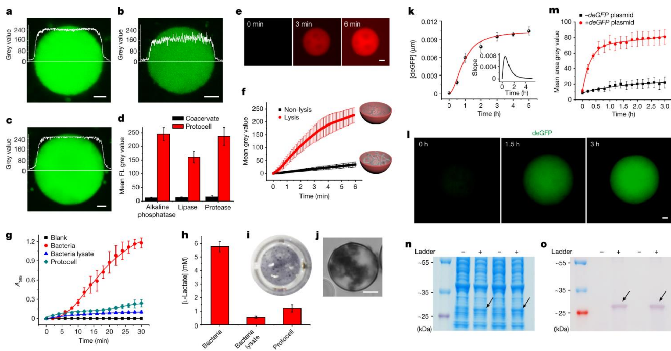
Fig. 3: Cytomimetic properties of bacteriogenic protocells. a–c , Confocal fluorescence microscopy images of single protocells containing bacterially derived alkaline phosphatase ( a ), lipase ( b ) or protease ( c ) recorded 30 min after exposure to cognate enzyme substrates showing intraprotocell production or sequestration of fluorescein ( a ) or BODIPY FL dye ( b and c ). d , The mean grey values for reactions shown in a–c and for the coacervate droplet controls. e , Time-dependent images of a single protocell after addition of resorufin- \beta -D-galactopyranoside (RBG), showing endogenous \beta -gal-mediated production of resorufin (red fluorescence). f , The mean grey values with time for resorufin formation in single bacteriogenic protocells (red) or single coacervate droplets with co-captured non-lysed bacteria (black) after addition of RBG. n = 3 . g , Formazan production (absorption at 565 nm ( A_{565} )) for native coacervate droplets (black), bacterial lysate (no droplets, blue), bacteriogenic protocells (green), and live E. coli and PAO1 cells (red). n = 3 . h , The final concentrations of l-lactate for the experiments shown in g ; n = 3 . i , A sample well containing formazan-containing protocells (purple dots) after glycolysis. j , A single bacteriogenic protocell 0.5 h after glycolysis with formazan in the interior. k , The time-dependent increase in deGFP concentration in bacteriogenic protocells undergoing endogenous in vitro gene expression. Curve is fitted to a Hill function ( t_{1/2} = 0.9 h, Hill coefficient = 2). Maximum expression rate is observed at 0.5 h (inset). n = 2 . l , The time-dependent increase in expressed deGFP (green fluorescence) within a bacteriogenic protocell. n = 3 . m , The corresponding time-dependent mean grey values for single protocells with (red) or without (black) the plasmid pEXP5-NT/deGFP. n,o , Gel electrophoresis profiles ( n ) and western blotting images ( o ) of extracted proteins after disassembly of protocells with (+) or without (–) the plasmid pEXP5-NT/deGFP. The arrows show an additional plasmid-dependent band at 27 kDa, which was stained by anti-GFP antibodies. Gel source data are provided in Supplementary Fig. 8. For a–c , e , j and l , scale bars, 5 \mu m. For f–h , k and m , data are mean \pm s.d.
