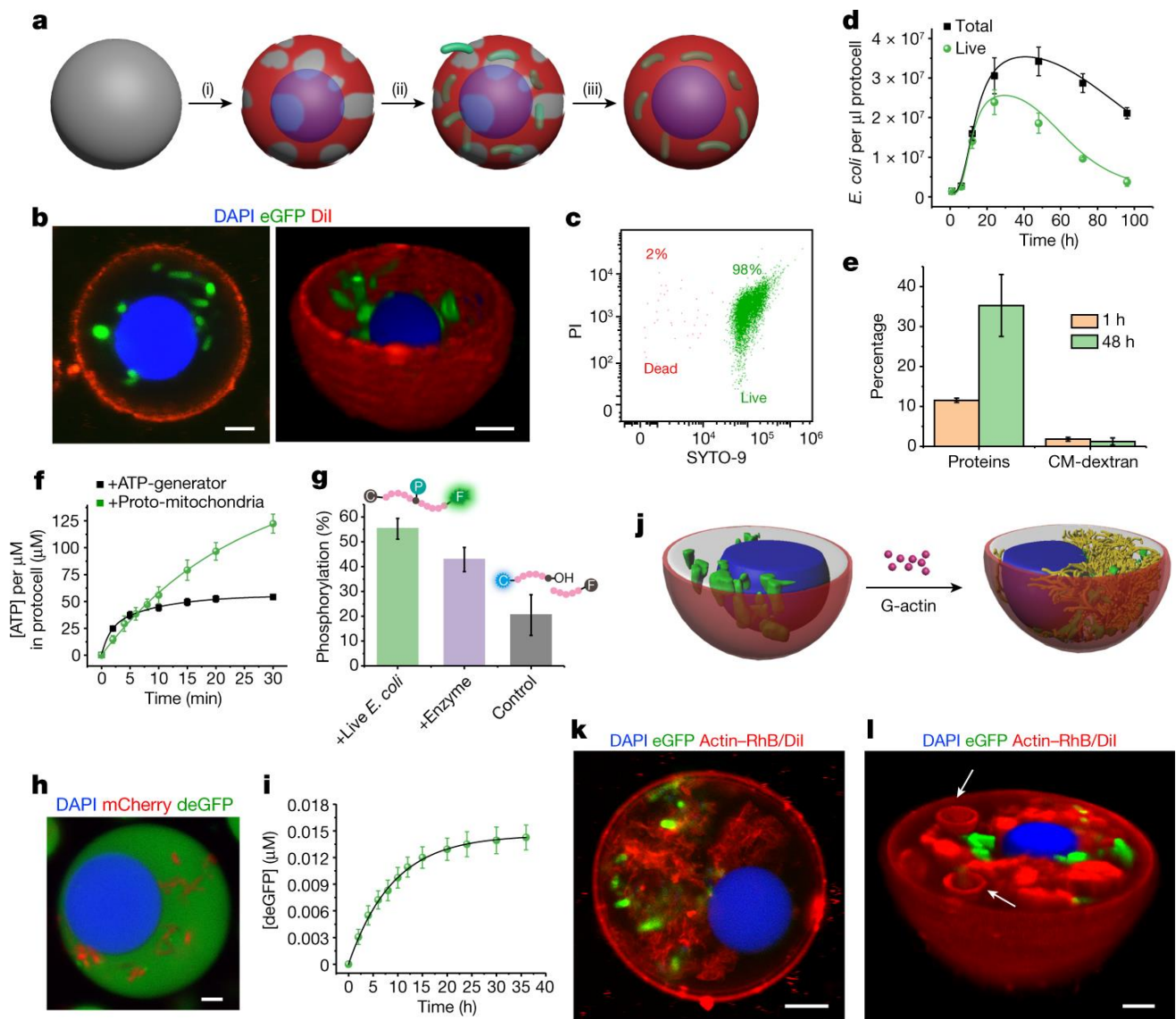
Fig. 5: Live-cell energization of bacteriogenic protocells. a , Implantation of live E. coli cells in bacteriogenic protocells. Construction of PDDA/UTP-based bacteriogenic protocells with a DNA–histone subcompartment and incomplete PAO1-derived membrane (i). Penetration of living E. coli and capture within the proto-cytoplasmic region (ii). Addition of PAO1-derived lipids and sealing of the protocell membrane (iii). b , 2D (left) and 3D (right) fluorescence images showing E. coli eGFP cells (green) in the proto-cytoplasmic regions of a single bacteriogenic protocell after membrane resealing (red). Blue, DNA–histone condensate. c , FACS live/dead analysis of bacteriogenic protocells containing SYTO-9/PI-stained E. coli cells. d , Time-dependent plots of the mean numbers of E. coli cells (total, black; live, green). e , Protein and CM-dextran levels in bacteriogenic protocells after incubation for 1 h (orange) and 48 h (green). f , Time-dependent plots of ATP concentration in bacteriogenic protocells by entrapped live E. coli cells (proto-mitochondria, green) or ATP-generation (PK–PEP–ADP pathway, black). g , Kinase activity in bacteriogenic protocells with entrapped live E. coli cells (green, 55%), encapsulated PK–PEP–ADP pathway (purple, 43%) or ATP control (bacterial lysate, grey column, 21%). h , In vitro gene expression of deGFP (green) in the proto-cytoplasmic region of a single hybrid protocell. Blue, DNA–histone subcompartment; red, entrapped live E. coli cells. i , deGFP expression over 40 h for a population of hybrid protocells. The exponential decay curve is shown ( [deGFP]_{max} = 0.015 \mu M , t_{1/2} = 9 h). j , F-actin assembly in bacteriogenic protocells containing ATP-generating live E. coli cells (green) and a DNA–histone proto-nucleus (blue). k , 2D image of a living/synthetic cell construct with F-actin microfilament
