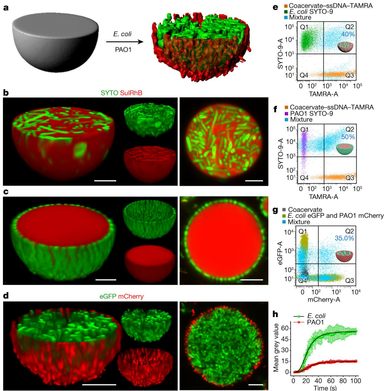
Fig. 1: Spontaneous capture of bacterial colonies in coacervate microdroplets. a , Specific uptake of live E. coli (green) and surface adsorption of PAO1 (red) cells in PDDA/ATP coacervate microdroplets. b–d , Confocal microscopy images of coacervate droplets after spontaneous capture of live E. coli ( b ), PAO1 ( c ) and a binary population of E. coli and PAO1 ( d ) cells. 3D (left) and 2D (right) fluorescence images are shown, with green/red fluorescence overlays, and filtered images. The fluorescence labels in b and c show coacervate (Sul-RhB, red) and bacteria (SYTO-9, green, DNA stain). The green and red fluorescence in d originate from expressed eGFP and mCherry. Scale bars, 5 \mu m. e–g , FACS fluorescence-gated analysis of the following coacervate microdroplet–bacteria mixtures: ssDNA–TAMRA-labelled droplets (orange), free SYTO-9-stained E. coli (green) and droplets with captured E. coli SYTO-9 (blue) ( e ); ssDNA–TAMRA droplets (orange), free SYTO-9-stained PAO1 (purple) and droplets with captured PAO1 SYTO-9 (blue) ( f ); non-fluorescent microdroplets (grey), free E. coli eGFP and PAO1 mCherry cells (olive green) and droplets with co-captured E. coli eGFP and PAO1 mCherry cells (blue) ( g ). For e and f , the quadrants comprise free E. coli (46%, gate Q1), free droplets (12%, Q3)
