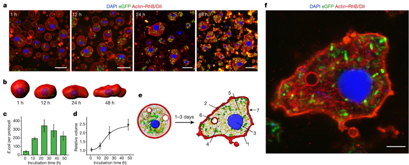
Fig. 6: Live-cell-mediated morphogenesis in bacteriogenic protocells. a , Time series of confocal fluorescence microscopy images of spherical bacteriogenic protocells with entrapped E. coli eGFP cells and F-actin (1 h) showing progressive transformation (12–48 h) into amoeba-like living/synthetic constructs due to on-site E. coli activity. Data were recorded at given time intervals from different populations. Red, F-actin and outer membrane; blue, DNA–histone condensate; green, guest live E. coli cells. b , Corresponding time series of 3D reconstruction images. The colours are as described in a . c , Time-dependent changes in the numbers of live E. coli cells per protocell. n = 3 . Data are mean \pm s.d. d , Time-dependent plot of relative volumes for single living/synthetic constructs. n = 3 . Data are mean \pm s.d. e,f , Diagram ( e ) and corresponding 2D confocal fluorescence microscopy image ( f ) of the functional protoliving synthetic cell with seven cytomimetic features: outer membrane (1); molecularly crowded proto-cytoplasm (2); membrane-free DNA–histone proto-nucleus (3); surrogate mitochondria ( E. coli cells) (4); proto-cytoskeleton (5); membrane-bounded spherical water vacuoles (6); and amoeba-like cell morphology (7). For a and f , scale bars, 10 \mu m.
