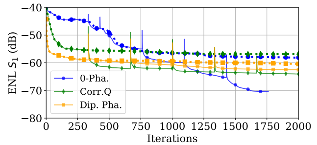
Fig. 5. Simulated horn antenna: ENL of the reconstructions on the first measurement sphere S_1 during a run of GS (dotted curves) and FiGS (plain curves) with nm -MT filter.
