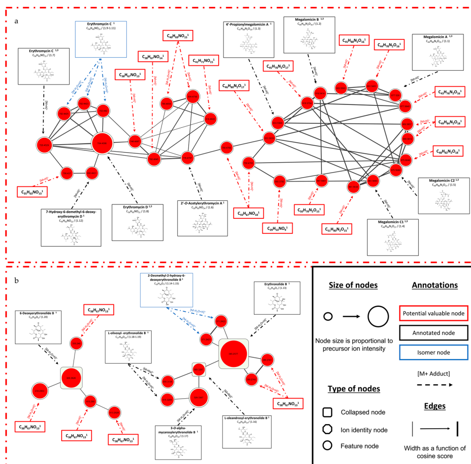
Figure 3. Main annotated clusters from the crude extract of Micromonospora fluostatini SH-82 (red node). (a) Main cluster representing the natural product class of erythromycins and (b) set of clusters representing the erythronolides family and derivatives. Superscript numbers in the annotations correspond to data from 1 SIRIUS, 2 GNPS or 3 ISDB timar bioinformatics tools. (The figure is in high definition, with the possibility of zooming-in).
