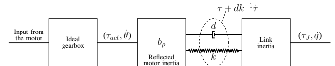
Fig. 2. Schematic diagram of a flexible robotic joint.
