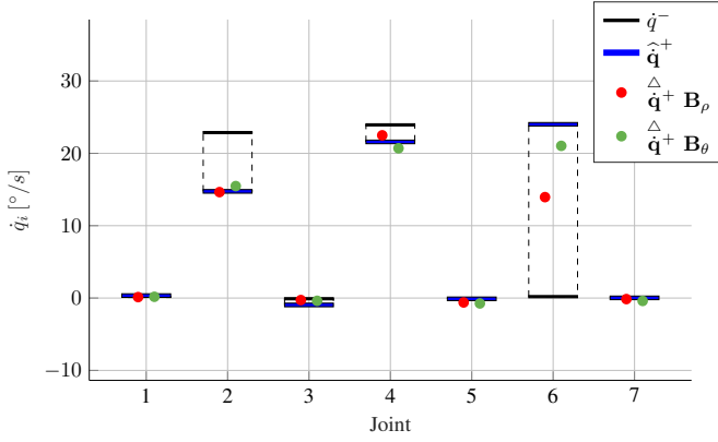
Fig. 5. Mean values of the virtual rigid-body post-impact velocity, \hat{\mathbf{q}}^+ (blue line), the measured ante-impact velocity, \dot{\mathbf{q}}^- (black line), and the predictions, \hat{\mathbf{q}}^+ , for joints 1 to 7 using either \mathbf{M}_\theta = \mathbf{M} + \mathbf{B}_\theta (green) or \mathbf{M}_\rho = \mathbf{M} + \mathbf{B}_\rho (red) (averaged over 5 experiments of type 1, see Table II).
