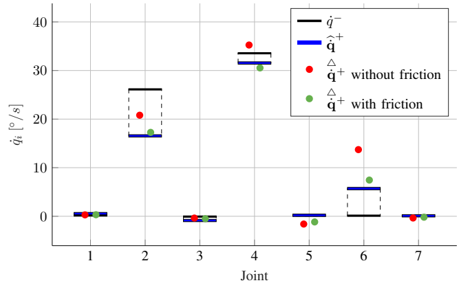
Fig. 6. Mean values of the virtual rigid-body post-impact velocity, \hat{\mathbf{q}}^+ (blue line), the measured ante-impact velocity, \dot{\mathbf{q}}^- (black line), and the predictions, \hat{\mathbf{q}}^+ , for joints 1 to 7 with (green) and without (red) considering tangential friction (averaged over 5 experiments of type 4, see Table II).
