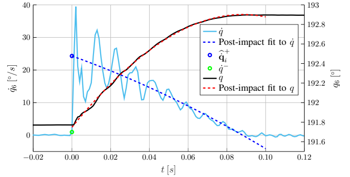
Fig. 4. Joint velocity of joint 6 for a representative impact experiment (type 1 in Table II), together with the joint position q (black line), post-impact polynomial fit and its derivative (dashed lines), and gross velocity jump estimation \hat{q}_i^+ .
