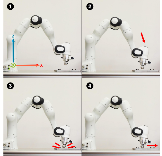
Fig. 1. Impact experiment example, recorded at Franka Emika: (1) The robot stands still at initial configuration; (2) The end-effector moves downwards and away from the robot base, as indicated by the red velocity arrow; (3) It impacts the steel plate; (4) After impact, it slightly bounces and then slides.
