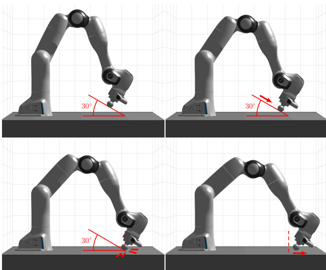
Fig. 2. Simulated impact scenario with an approach angle of 30 degrees and an impact velocity of 0.1 m/s. Time evolves from left to right, and from top to bottom. The impact location is indicated by the vertical dashed line.
