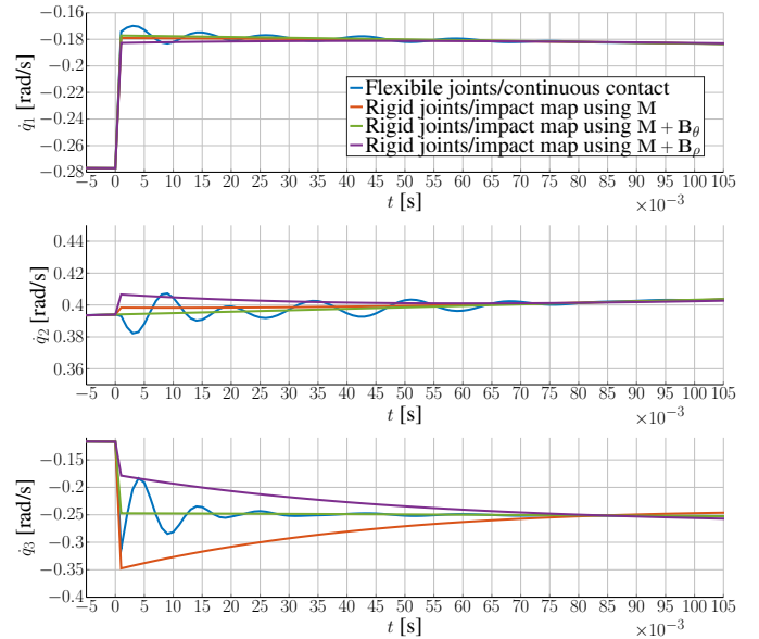
Fig. 3. Comparison of the post-impact joint velocities for a flexible-joint robot with a continuous contact model and three instances of a rigid-joint robot with different inertia matrices for the impact map (impact as in Figure 2). Results obtained with \mathbf{M} + \mathbf{B}_\theta yield the best asymptotic behaviour w.r.t. the flexible joints + continuous contact model which serves as a reference.
