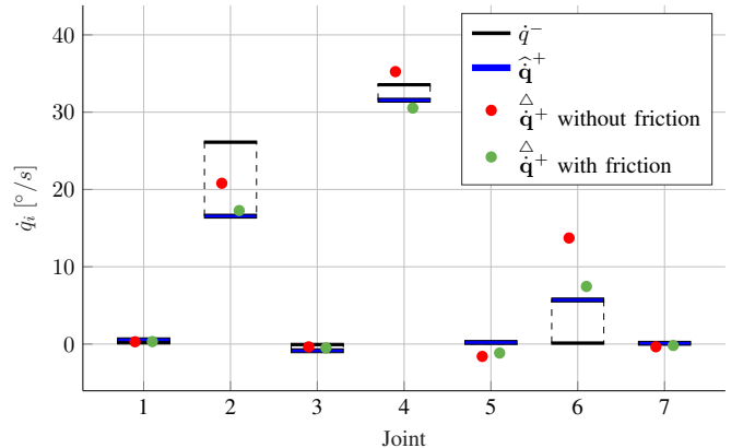
Fig. 6. Mean values of the virtual rigid-body post-impact velocity, \hat{q}^+ (blue line), the measured ante-impact velocity, \dot{q}^- (black line), and the predictions, \hat{q}^+ , for joints 1 to 7 with (green) and without (red) considering tangential friction (averaged over 5 experiments of type 4, see Table II).
