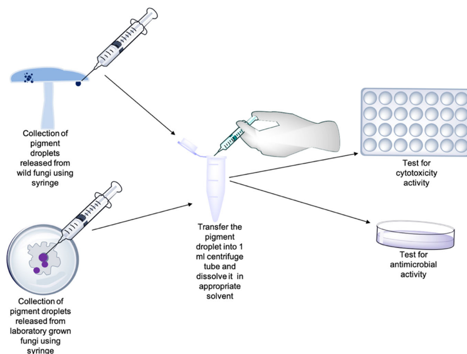
Figure 3. Isolation of concentrated pigment droplets (authors' unpublished data) released by fungi on their mycelia surfaces and testing them directly for biological properties in a simple and rapid way. Before or after confirming the bioactivity, these pigment droplets can be purified with TLC as shown in Figure 2.
