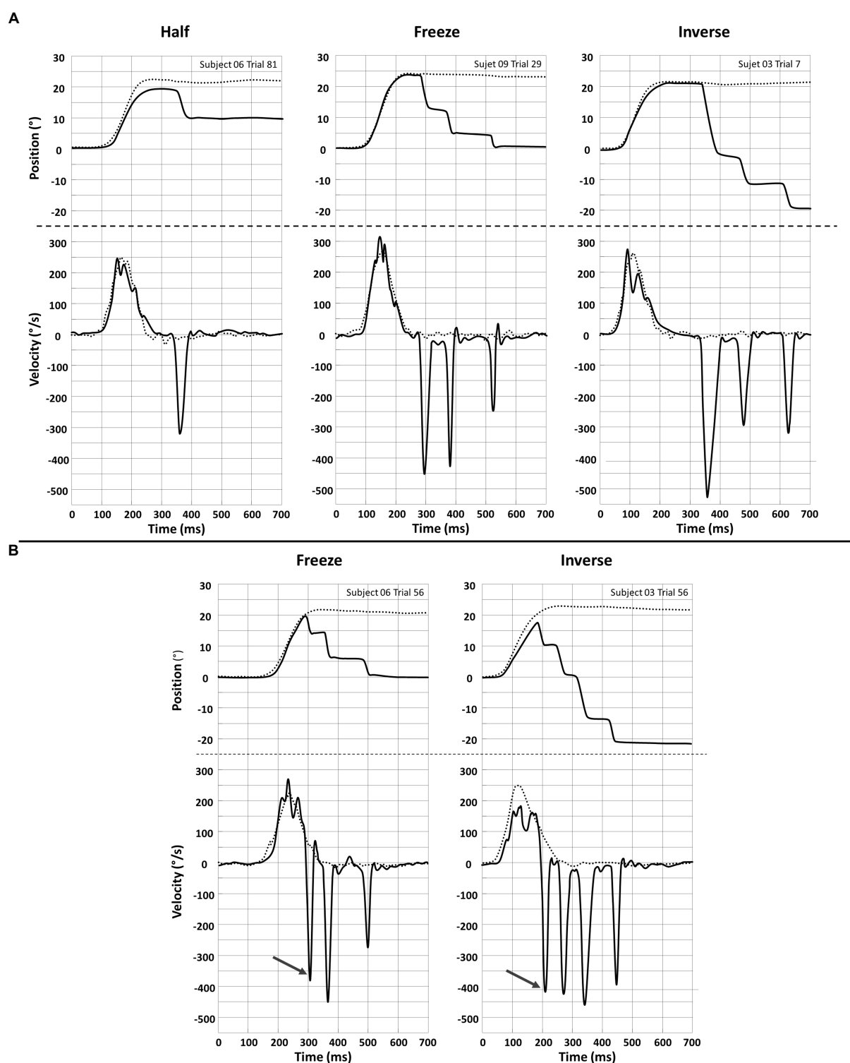
FIGURE 6 Recording of Head (—) and eye (---) position (upper plots) and velocity (lower plots) for a single head impulse in the Half, Freeze and Inverse VR setting. Eye positions are inverted in the plot by convention. (A) Responses with overt saccades only. (B) Responses with a covert saccade (arrow) preceding overt saccades.
