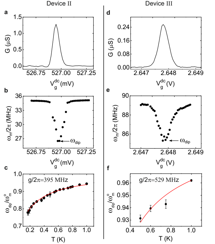
Fig. S13: Strong anharmonicity and ultra-strong coupling regime in two other devices. (a,b) Conductance and mechanical resonance frequency as a function of gate voltage at 170 mK for Device II. (c) Suppression of the resonance frequency as a function of temperature at the conduction peak. The solid red line is the SET-base prediction. (d,e) Conductance and mechanical resonance frequency as a function of gate voltage at 6 K for Device III. (f) Suppression of the resonance frequency as a function of temperature at the conduction peak.
