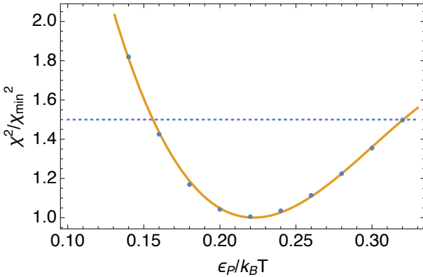
Fig. S6: Dependence of the \chi^2 on \epsilon_P/k_B T .
