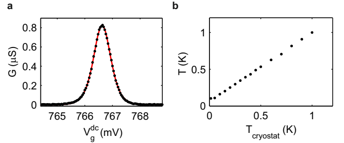
Fig. S8: Temperature calibration. (a) Gate voltage dependence of the conductance of device I at T = 1 K. The red solid line is the fit to the data using Eq. 75. (b) The electron temperature of the device measured as a function of the cryostat temperature.
