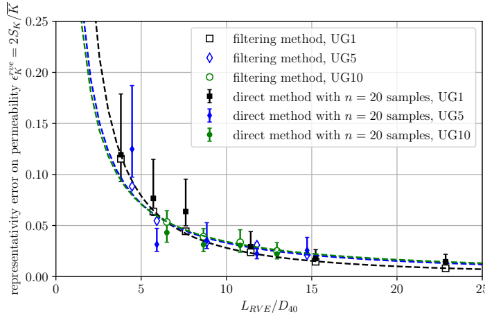
Fig. 18 Representativity error \epsilon_K^{\text{rve}} estimated with a 95% confidence interval by the direct and filtering methods for the three types of gradation, as a function of the sample size L_{\text{RVE}} scaled by the particle diameter D_{40} . Dotted lines: power-law fits of median values given by the filtering method.
