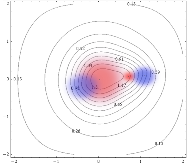
b Without dark matter and without kappa renormalization but with the densities Figs. a+c
