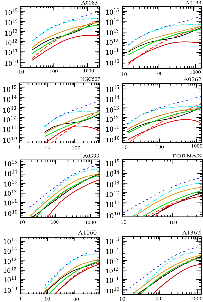
Figure 3 Plot of the radial mass profile for clusters of the sample in Table 1. For the caption see the Figure 1. The solid red curve displays the \kappa -model dynamic mass, with a non-isothermal temperature profile of \alpha = 2 .
