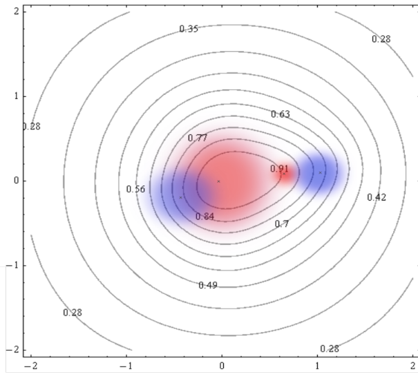
a Without dark matter and without kappa renormalization but with the densities Figs. a+b
