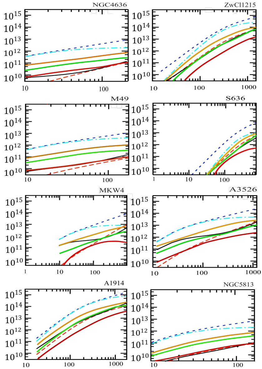
Figure 3 Continued galaxy cluster mass profiles
