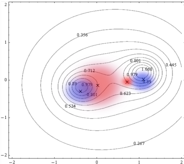
c Dark matter
