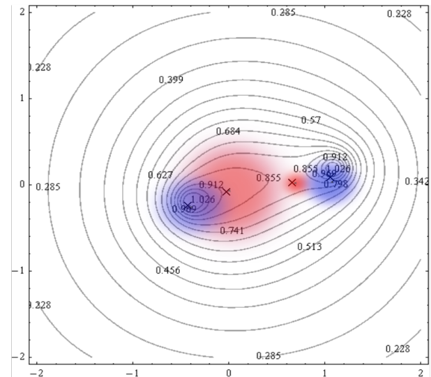
d kappa model
