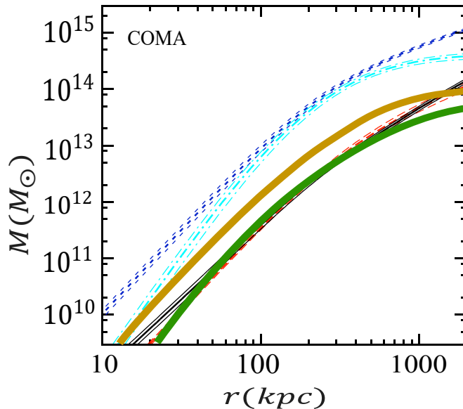
Figure 1 COMA cluster profile. The horizontal axis is the radius in kpc and the vertical axis is mass in units of the solar mass M_\odot . The red long dashed curve is the ICM gas mass derived from X-ray observations (compilation of Reiprich, 2001; Reiprich and Böhringer, 2002); the short dashed blue curve is the Newtonian dynamic mass; the dashed-dotted cyan curve is the MOND dynamic mass; the solid black curve is the MSTG dynamic mass (Brownstein and Moffat, 2006). Our contribution is displayed as the amber curve, showing the \kappa -model dynamic mass with the temperature T = 8.38 keV. The solid green curve displays the \kappa -model dynamic mass, assuming a non-isothermal temperature profile with \alpha = 1 in eq. 8.
