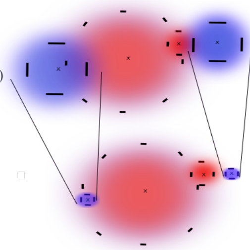
Figure 6 Basic illustration of the combined action of both gravitational and kappa lensings. The lensing by the hot gas is used as a reference for the two figures a and b.
