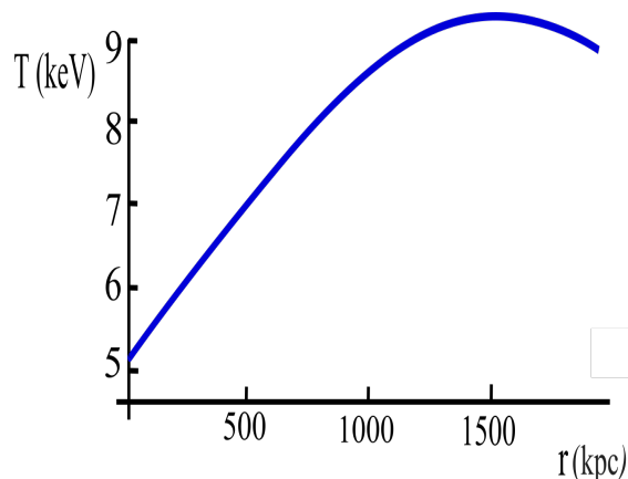
Figure 2 Predicted mean temperature profile in the COMA cluster in the framework of the \kappa -model
