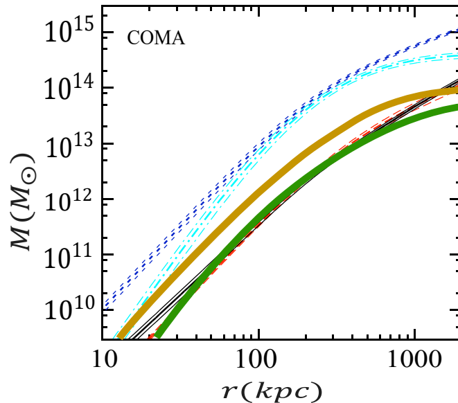
Figure 1 COMA cluster profile. The horizontal axis is the radius in kpc and the vertical axis is mass in units of the solar mass M_\odot . The red long dashed curve is the ICM gas mass derived from X-ray observations (compilation of Reiprich, 2001; Reiprich and Böhringer, 2002); the short dashed blue curve is the Newtonian dynamic mass; the dashed-dotted cyan curve is the MOND dynamic mass; the solid black curve is the MSTG dynamic mass (Brownstein and Moffat, 2006). Our contribution is displayed as the amber curve, showing the \kappa -model dynamic mass with the temperature T = 8.38 keV. The solid green curve displays the \kappa -model dynamic mass, assuming a non-isothermal temperature profile with \alpha = 1 in eq. 8.
