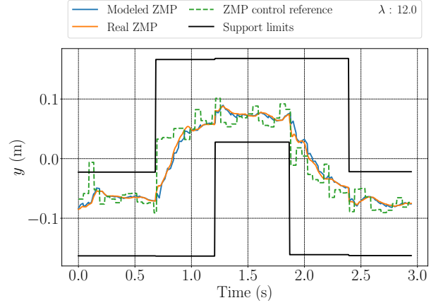
(a) On HRP-2KAI.
