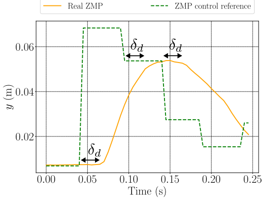
Fig. 11: Delay between the real ZMP and the sent reference on HRP-2KAI.
