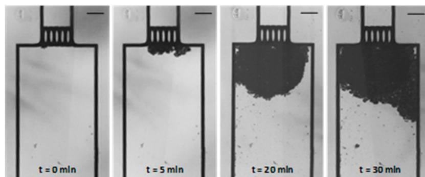
Figure 2. Pictures of the microchannel during the filling procedure at different times. The scale bar is 100 \mu\text{m} .
