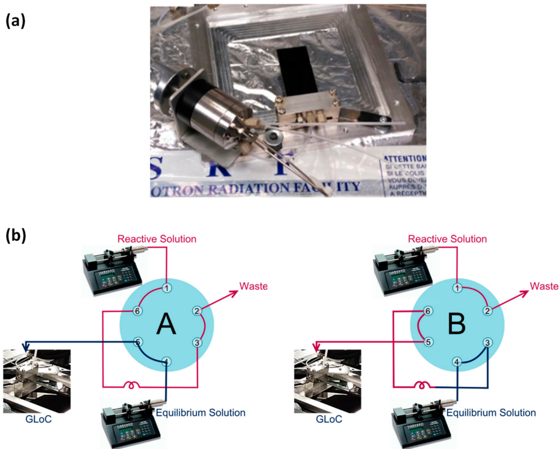
Figure 3. (a) Image of the experimental set-up used at ESRF including a 6-valve port for the injection of a known volume of the reactive solution and the silicon-Pyrex microreactor with its associated compression part for injecting the fluids. (b) Typical experimental procedure allowing the loading of reactive solution into a loop (position A, left), while the saturated (equilibrium) solution flows through the microreactor, before its injection into the 3D porous medium (position B, right).
