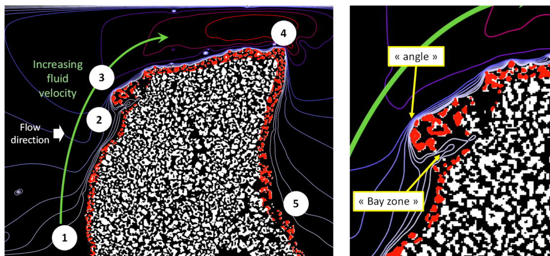
Figure 8. Section of the computational domain for geometry 19 with the solid phase in white, the part that will be dissolved during reactive percolation between 19 and 20 (approximate registration) in red and the velocity modulus isovalue lines (from the light grey line on the bottom to the red line on the top: 0.01, 0.015, 0.02, 0.03, 0.04, 0.05, 0.1, 0.15, 0.20 \text{m}\cdot\text{s}^{-1} ).
