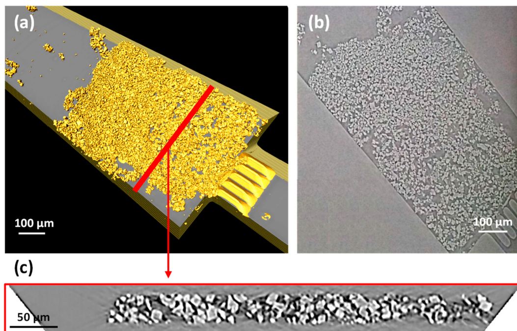
Figure 4. (a) 3D reconstruction of the model packed bed porous medium, (b) 2D Y-Z image of the microreactor filled with a \text{CaCO}_3 particle packed bed, (c) cross section view of the filled microreactor displaying the packing of the \text{CaCO}_3 particle in the z dimension along the red line in Figure 4a.
