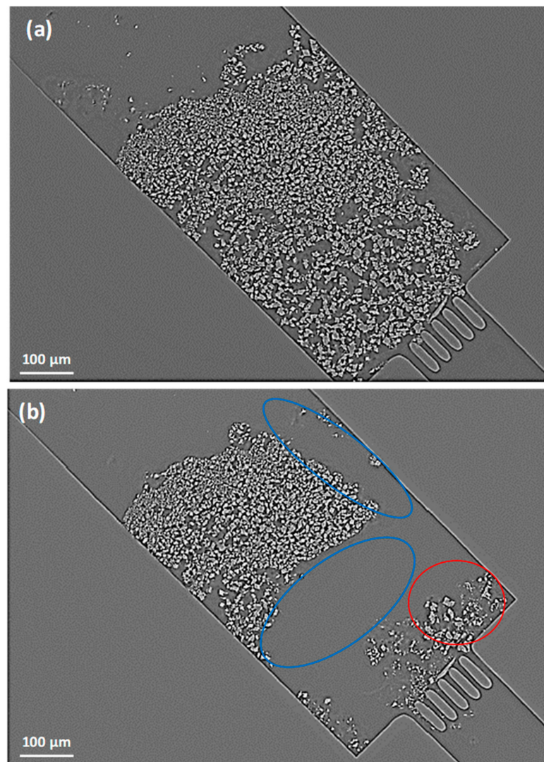
Figure 5. 2D X-rays images of the model 3D packed bed porous medium taken after (a) 3 injections and (b) 17 injections. Local preferential dissolution of the packed particles are highlighted in the blue circles, while displacement of non-dissolved particles can be seen in the red circle.
