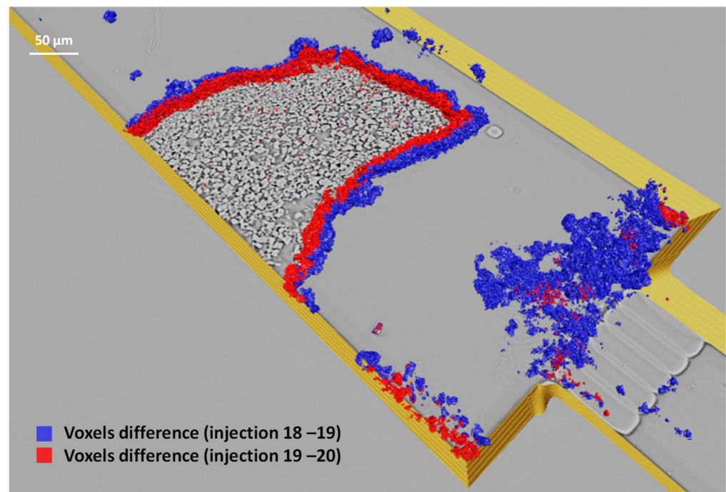
Figure 6. Superposition of 3D images of the packed bed porous medium taken between injections 18, 19, and 20, showing the dissolved materials. The blue and red colored \text{CaCO}_3 particles correspond to the volume variation (in voxels) of the packed bed between injections 18 and 19, and 19 and 20, respectively.
