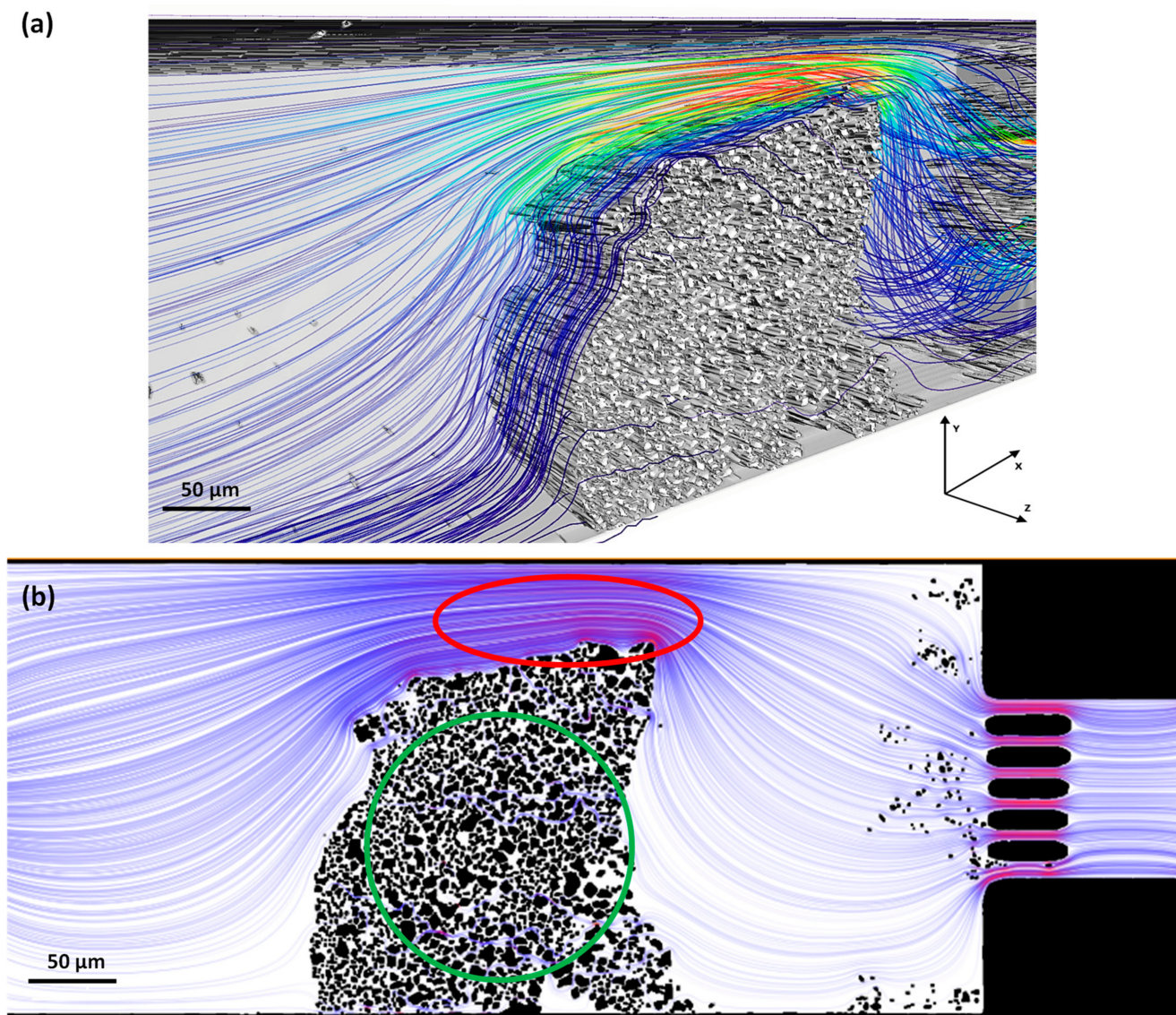
Figure 7. (a) Calculated 3D fluid flow pattern inside the packed bed porous medium after injection number 19 and (b) 2D view at half depth with additional green and red circle highlighting the different fluidic behaviors in the porous medium and around the porous medium, respectively.
