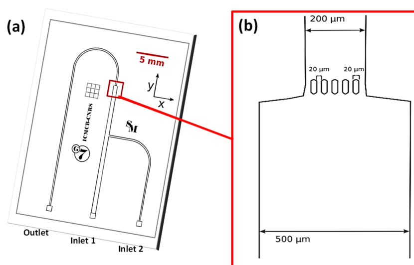
Figure 1. (a) Scheme of the microreactor design. (b) Enlarged view of the microfilter section.
