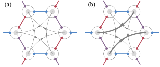
FIG. 2. Chiral amplitudes in the Kitaev model from the Majorana mean-field theory. In (a) we show the NNN chiral Majorana amplitudes, \langle c_i c_j \rangle , induced in the ground state MMFT wave function either by a magnetic field perpendicular to the plane, t = 1 , or a DM vector oriented perpendicular to the plane ( d = 1 ). These are responsible for the chiral QSL with Chern number \nu = +1 ( \text{GQSL}_{+1} ) discussed in the text. (b) Anisotropic amplitudes (the thickness corresponds to the different strength) arising from finite DM d \neq 1 (with no applied magnetic field) responsible for the opening of the gap for 0.5 < D < 0.65 (with K = 1 and d = 0 ) in the \text{GQSL}_{\pm 1} . The snapshots show one of the two possible chiralities of the ground state ( \nu = +1 ). Note that (a) and (b) amplitudes are smoothly connected as shown in the phase diagram of Fig. 1.
