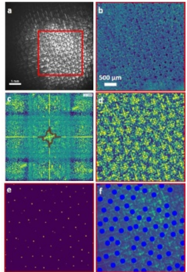
FIG. 8. Intermediary steps produced by the FFT centers identification method: (a) raw image ; (b) dispersion image; (c) FFT of the dispersion image; (d) Inverse Fourier Transform of the image with just the low frequencies inside the brown contour of c; (e) binary image representing the tip of the dendrites from applying a threshold on (d); (f) centers and segmentation superimposed to the raw image. The red squared region in a is represented in b, d, e and f.
