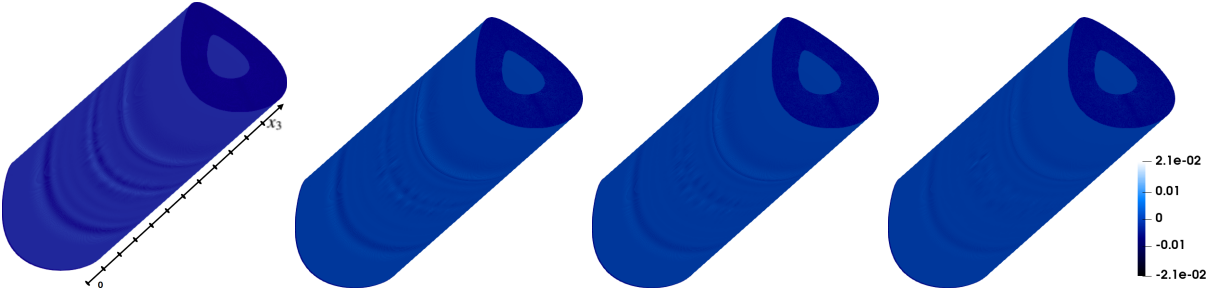
FIGURE 8. \tilde{E}_3^\delta with \delta = 0.15, \delta = 0.1, \delta = 0.075, \delta = 0.05 at T = 6 .
