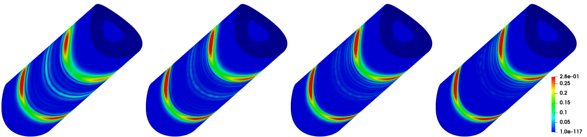
Figure 6. |\tilde{E}_T^\delta| with \delta = 0.15 , \delta = 0.1 , \delta = 0.1 , \delta = 0.075 at T = 6 .
