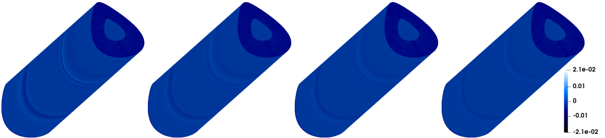
Figure 9. \widetilde{E}_3^{\delta,2} with \delta = 0.15, \delta = 0.1, \delta = 0.075, \delta = 0.05 at T = 6 .
