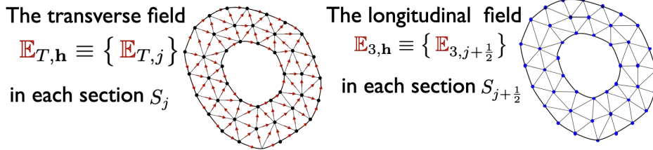
Figure 1. Two types of degrees of freedom.
