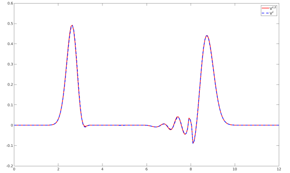
Figure 5. The voltages V^\delta (in blue) and V^{\delta,2} (in red) at T = 6 .
