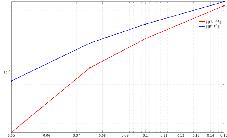
Figure 11. In blue: \|E^\delta - E^0\| . In red: \|E^\delta - E^{\delta,2}\| , for T = 6 . (On the "loglog" scale).
