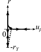
Figure 9: The considered brittle constitutive behavior, as an impulse/displacement jump relationship (the dotted line denotes a brutal jump in the status)
