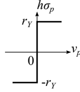
Figure 2: The considered constitutive behavior, as an impulse/velocity jump relationship
