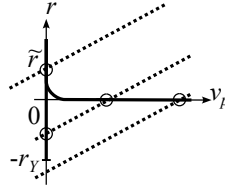
Figure 10: The brittle fracture solution as the intersection of the impulse/velocity behavior (plain line) and the reduced dynamics (dotted line)
