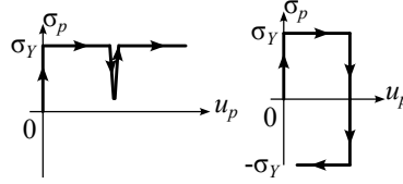
Figure 3: The considered constitutive behavior, as a stress/displacement jump relationship
