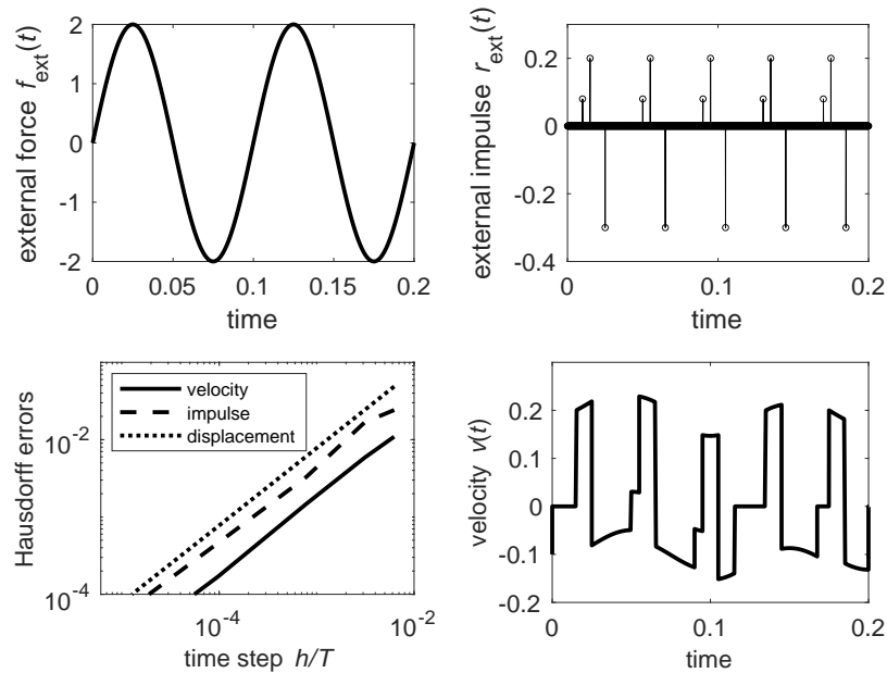
Figure 15: The loading with forces and impulses, the numerical convergence of the solution with respect to time discretization and the reference solution for velocity
