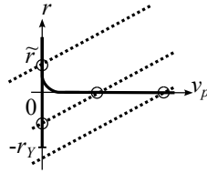
Figure 8: The brittle fracture solution as the intersection of the impulse/velocity behavior (plain line) and the reduced dynamics (dotted line)
