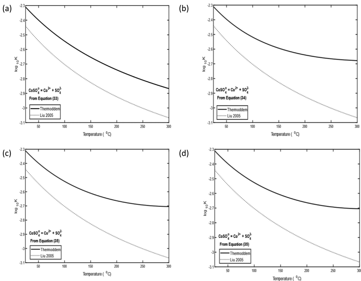
Fig. 10. Extrapolation of \log(K_{i,T}) for \text{CoSO}_4^0 \rightleftharpoons \text{Co}^{2+} + \text{SO}_4^{2-} with thermodynamic data from 2 different sources [1,49] using (a) van't Hoff, (b) "Cp approximation", (c) Density and (d) Unexpanded HKF models.
