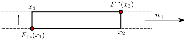
Fig. 1. The “frame” configuration for the regularized light ray operator: long sides are stretched along the light ray with the direction n_+ , short sides oriented in an orthogonal direction.
