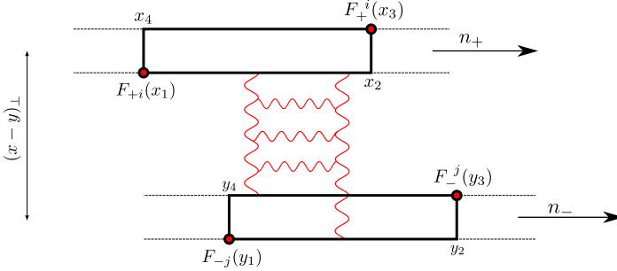
Fig. 2. Two Wilson frames, at a distance |x - y|_\perp from each other, stretched in two different light-cone directions n_+ and n_- and a typical gluon exchange between them.
