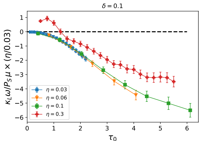
FIG. 8. Single parameter scaling of the normalized angular momentum leak for \eta = 0.03 , \eta = 0.06 , \eta = 0.1 and \eta = 0.3 obtained by multiplying them by \eta/0.03 . For \eta = 0.3 , the scaling starts to break down. This figure shows that for values of \eta up to 0.1, the total radiated angular momentum is proportional to the mean free path \ell_0 times f(\tau_0) \sim \tau_0^2 for \tau_0 \leq 2 .
