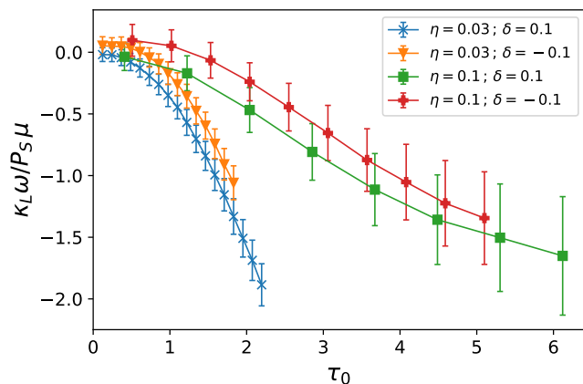
FIG. 7. Impact of opposite detunings on the total AM leakage for the curves \eta = 0.03 and \eta = 0.1 . The bars indicate the standard deviation of the distribution of \kappa_L\omega/P_S\mu values.
