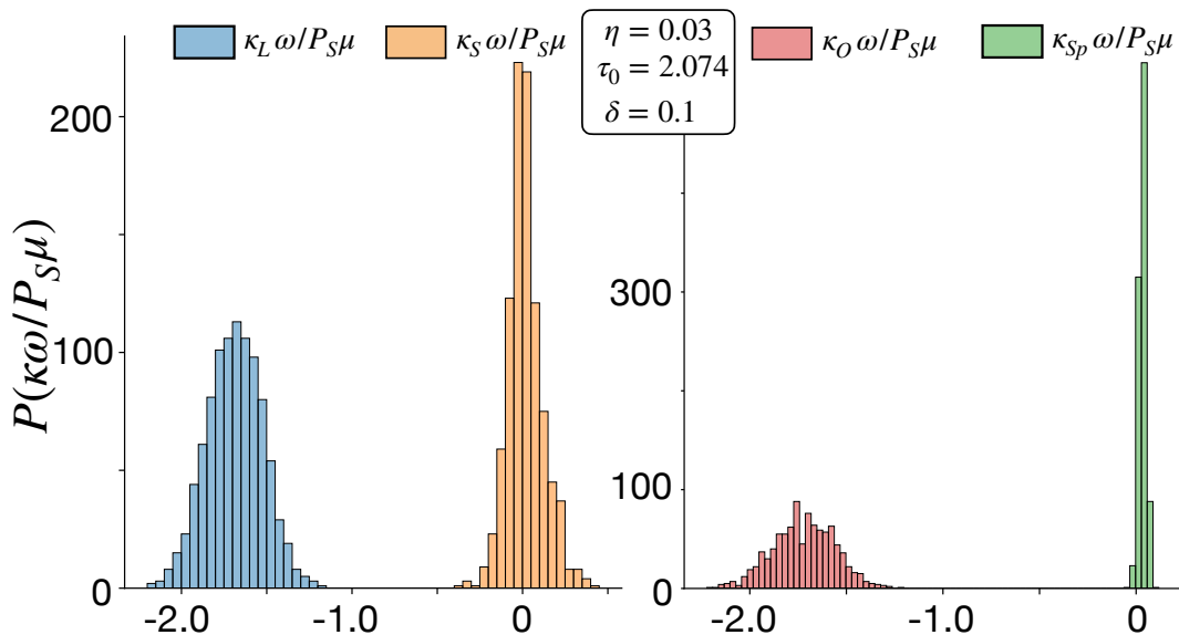
FIG. 6. Left: the distribution of the normalized total leakage \kappa_L\omega/P_S\mu and the normalized torque on the source \kappa_S\omega/P_S\mu for \eta = 0.03 , optical thickness \tau_0 = 2.074 and detuning \delta = 0.1 . The right figure depicts the distribution of the normalized source leakage \kappa_{Sp}\omega/P_S\mu and the normalized \kappa_O\omega/P_S\mu for the same values of \eta , \tau_0 and \delta .
