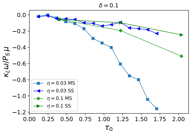
FIG. 5. Effect of multiple scattering on the radiated optical AM. The multiple scattering curves are labelled 'MS' and the single scattering approximation curves are labelled 'SS'.
