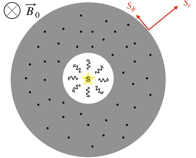
FIG. 1. Schematical picture of the geometry considered in this work. An unpolarized dipole source is located at the origin, surrounded by two shells: the first shell is empty to avoid scattering close to the source, while the second shell contains an on average homogeneous dipole gas. The external magnetic field is directed perpendicular to the plane. The electromagnetic Poynting vector exhibits an azimuthal component \mathbf{S}_\phi which is orthogonal to both the magnetic field and the radial vector. This component induces the emission of angular momentum into space.
