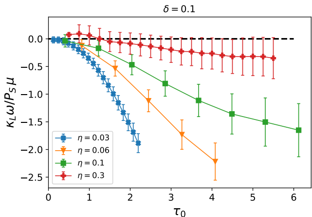
FIG. 2. Numerical results for the total leakage \kappa_L\omega/P_S\mu per emitted photon for different values of the parameters \eta and \tau_0 . The bars indicate the standard deviation of the full statistic of \kappa_L values, and are not error bars. The dashed line denotes the level zero.
