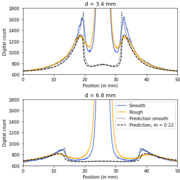
Figure 7. Profiles for each thickness, the black lines are modelled respectively through equation (1) for the smooth interface, and equation (7) for the rough one.
