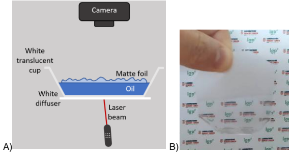
Figure 5. A) Scheme of the setup. B) Picture of the matte lamination foil, the bottom part is covered by oil.
