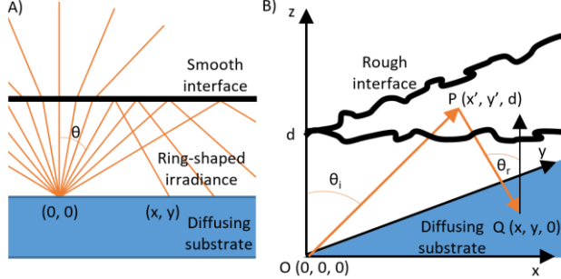
Figure 2. A) Internal reflections inside the coating layer for a smooth interface. B) Scheme of the system for a rough interface.
