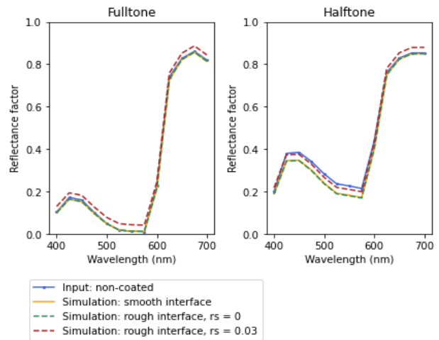
Figure 8. Modelling of the effect of matte and glossy coatings on the reflectance factor of magenta prints.
