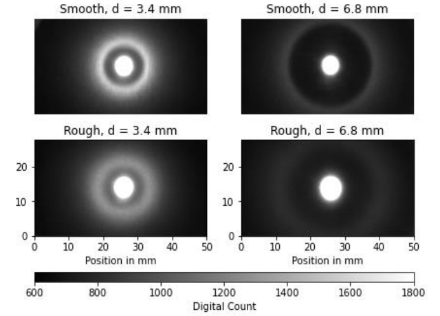
Figure 6. Pictures of the halo induced by a smooth and a rough interface with air for two different coating thicknesses.
