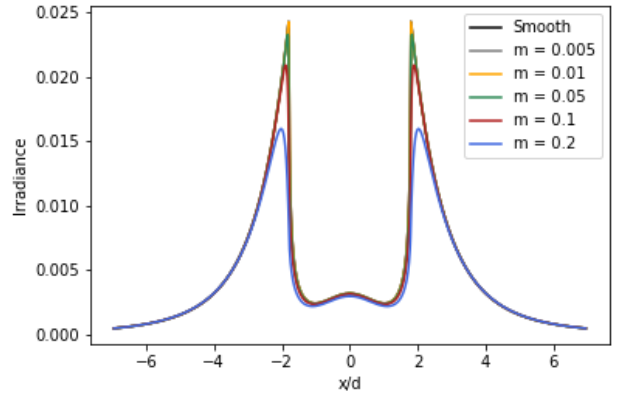
Figure 3. Profiles of the modelled halos, with an initial exitance at the central point equal to unity.
