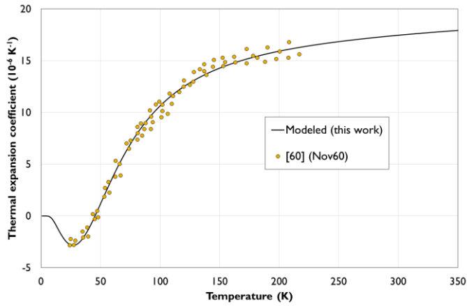
Fig. 3. Experimental and assessed thermal expansion of \alpha -Sn
