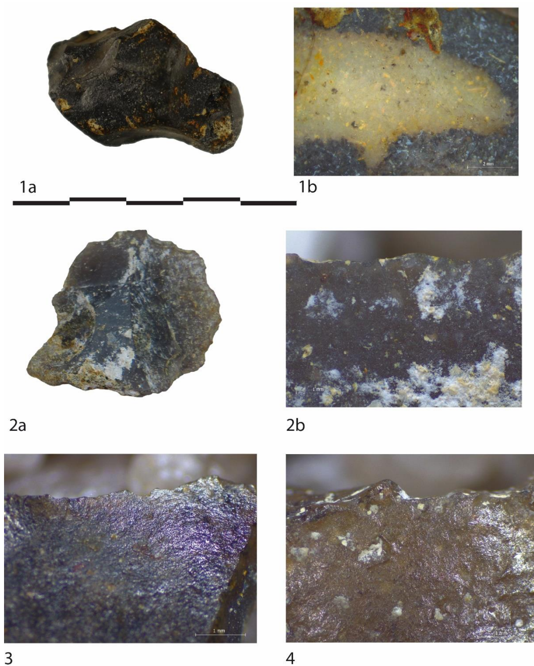
Figure 12. Macro- and micro-photos of lithic material of layers F, I1 and G.
