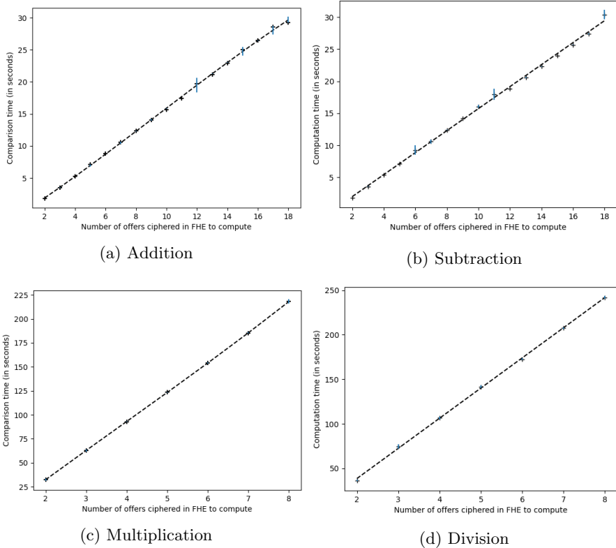
Fig. 9: Computation time according to the number of ciphred numbers submitted
