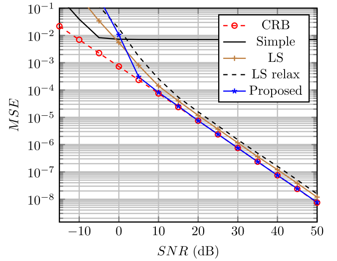
(b) MSE versus SNR (N = 10 samples).
