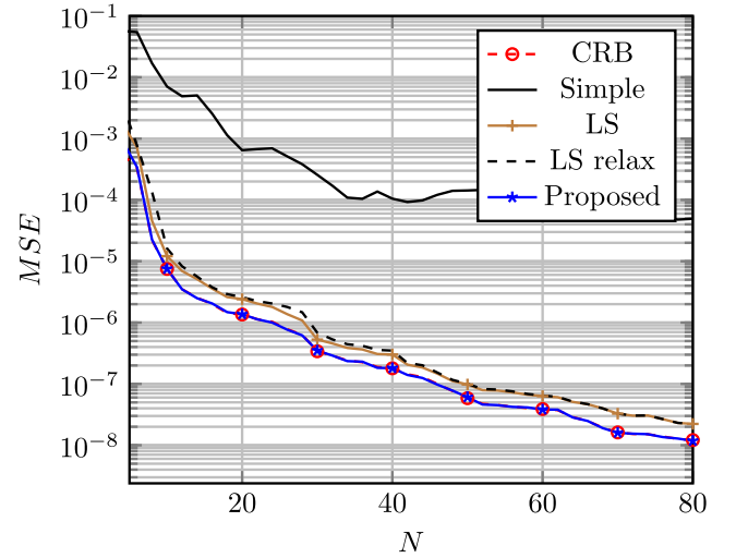
(a) MSE versus N (SNR = 20 dB)
