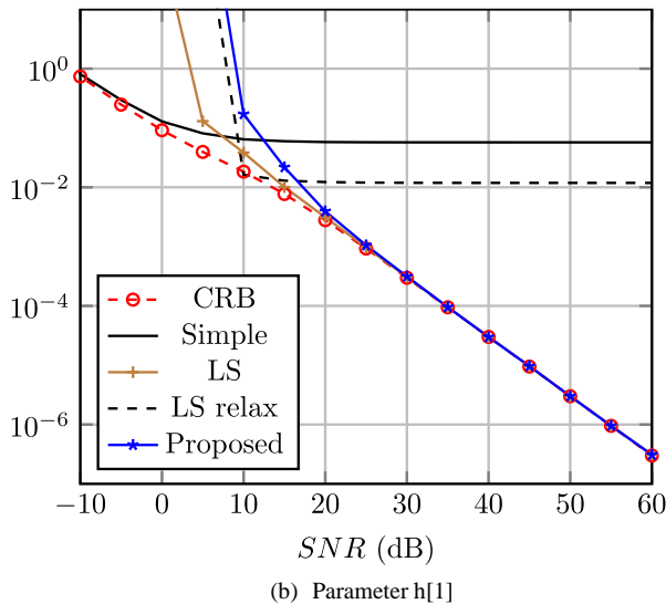
Figure 4: Estimation of the FIR parameters versus SNR ( N = 20 samples, FIR parameters: [1, 0.992 + 0.243j, 0.182 - 0.516j] )
