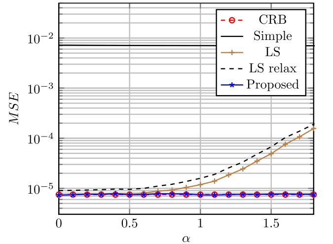
(c) MSE versus receiver impairment magnitude \alpha ( \nu_r(\alpha) = \alpha \nu_r , N = 10 samples, SNR = 20 dB).
