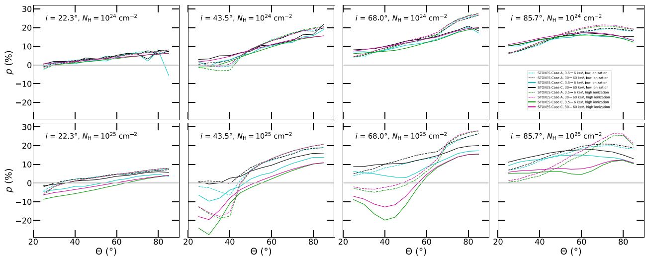
Figure 5. The same as in Fig. 4, but energy-averaged polarization degree, p , versus half-opening angle \Theta is shown for i = 22.3^\circ , i = 43.5^\circ , i = 68.0^\circ , and i = 85.7^\circ (left to right). In different view of the results, we see the polarization dependence on half-opening angle: the smaller the vertical extension of the torus is, the more equatorial reprocessing we witness and the higher and clearer the parallel polarization contribution is, especially for low column densities.
