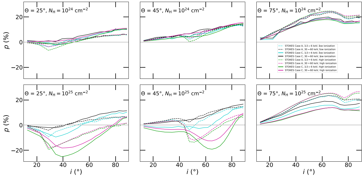
Figure 4. The same as in Fig. 3, but energy-averaged polarization degree, p , versus inclination i is shown. The reprocessed polarization can reach tens of per cent and geometrical details are important. For lower densities, the prevalent polarization orientation is parallel with the axis of symmetry. Circular tori (Case C) then in some cases of high obscuration lead to a resulting perpendicular polarization.
