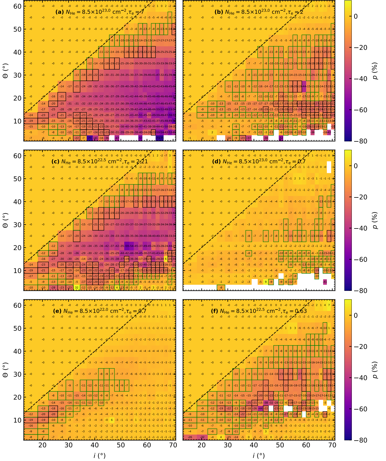
Figure A5. The same as in Fig. 11, but for a Case B elliptical obscurer with b = R/8 . The two branches of solutions in the displayed configuration space remain in the same topology as in Fig. 11.
