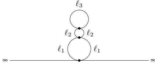
FIGURE 1. An example of a “tower of bubbles” graph. Each of these graphs, identified in Example 2.4 of [6], is built of a real line and a finite sequence of two-by-two tangent circles.
