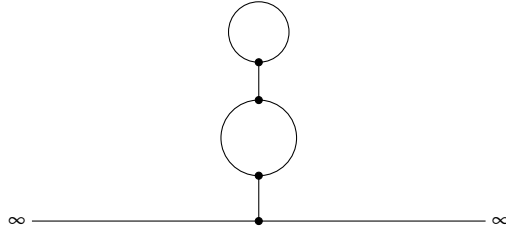
FIGURE 8. A graph with \#F(\mathcal{G}) = 2 where nodal ground states never exist, independently of the length of the edges.
