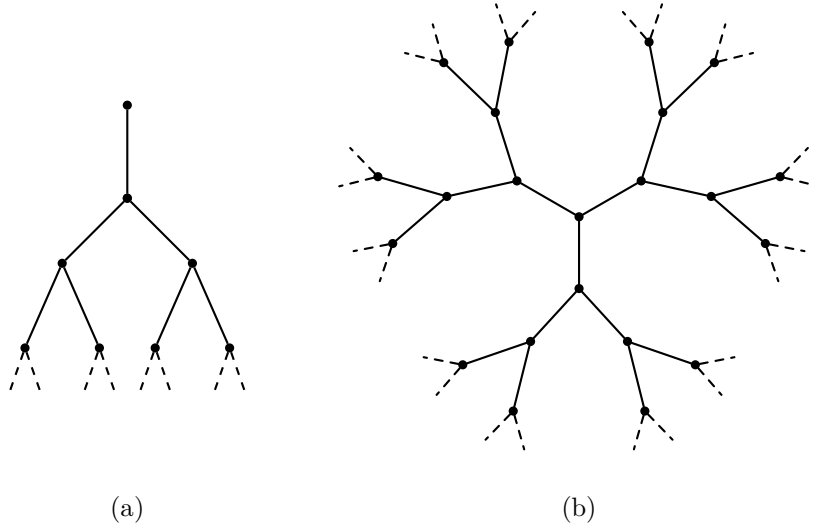
FIGURE 3. Examples of a rooted tree (a) and an unrooted tree (b).
