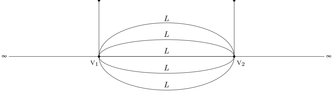
FIGURE 9. The graph \mathcal{G}_{N,L} with N = 5 .
