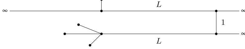
FIGURE 6. Example of a graph \mathcal{G}_L as in Theorem 4.15, constructed starting with two graphs in Figure 5. If the vertical edge on the right is sufficiently far from the pendants of the graph, nodal ground states exist.
