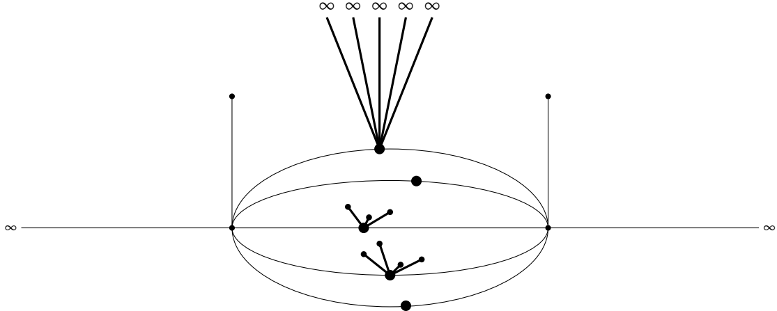
FIGURE 10. Example of a graph as in Theorem 1.9 hosting a nodal ground state whose nodal set (thick on the picture) is made of two isolated points, two groups of three line segments and a group of five half-lines.
