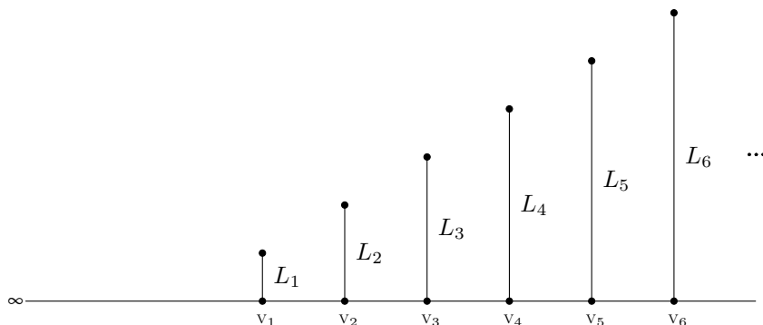
FIGURE 4. The graph \mathcal{G} described in Remark 4.6.
