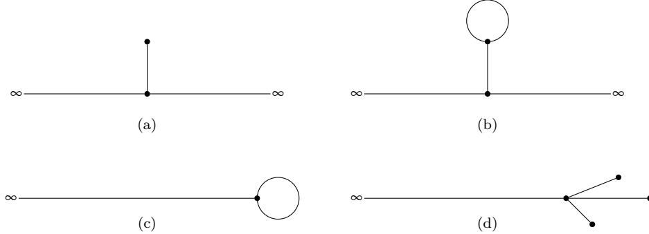
FIGURE 5. Some graphs with Z = \emptyset admitting ground states. (a): line with a pendant; (b): signpost; (c): tadpole; (d): 3-fork.
