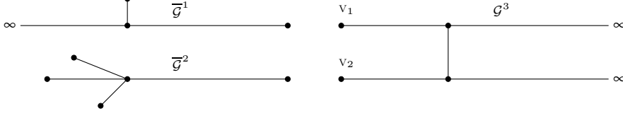
FIGURE 7. The graph \mathcal{G}_L of Figure 6 splits into the three graphs \overline{\mathcal{G}}^1 , \overline{\mathcal{G}}^2 and \mathcal{G}^3 .
