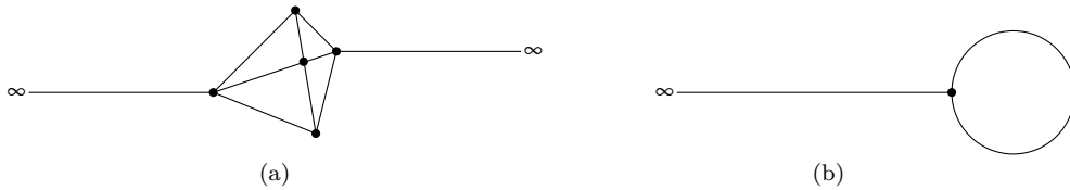
FIGURE 2. Examples of graphs with half-lines satisfying \#F(\mathcal{G}) = 0 (a) and \#F(\mathcal{G}) = 1 (b).
