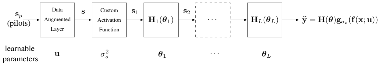
Fig. 1: Proposed ParamNet network architecture. The network is composed of a data augmented layer, \mathbf{f}(\cdot; \mathbf{u}) , a non-linear activation function, \mathbf{g}_{\sigma_s}(\cdot) , and L linear layers \mathbf{H}_l(\boldsymbol{\theta}_l) modeling the hardware impairments and channel effects.
