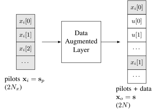
Fig. 2: Illustration of the Data Augmented Layer. The learnable parameters correspond to the data \mathbf{u} = [u[0], u[1], \dots]^T .
