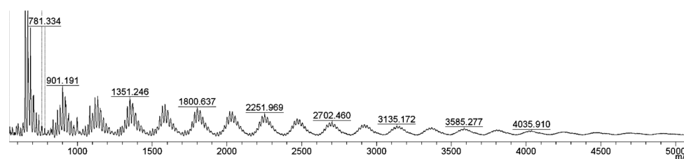
Figure 4. MALDI MS spectrum of poly(Cys-Met), positive ionization.
