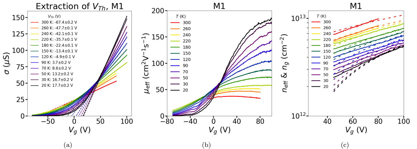
FIG. 3: (a) Conductivity versus gate voltage of device M1 (as in Fig. 3.a of the main text) between 300 K and 20 K, showing the linear fit (in dashed lines) used to extract a temperature dependent V_{Th} . (b) Effective mobility \mu_{eff} = (\partial\sigma/\partial V_g)/C_{ox} versus gate voltage for the same measurements. (c) Carrier density versus gate voltage obtained from the previous analysis in (a) and (b), n_{eff} is in full lines and n_g is in dashed lines.
