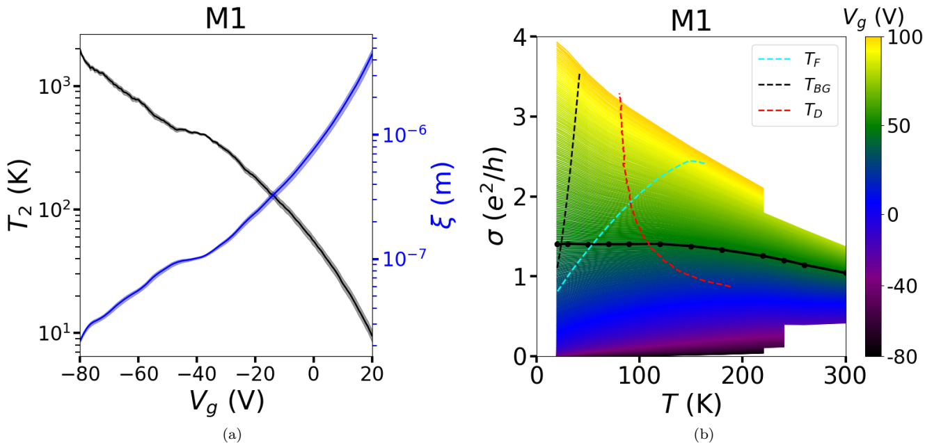
FIG. 6: (a) Computed localization length ( \xi ) and extracted Efros-Shklovskii activation temperature ( T_2 ) for M1 device. (b) Conductivity of device M1 in units e^2/h . The colored dashed lines show the limits of validity of a QPT arising purely from electronic effects. The solid black line is the curve used to scale the data into two branches.
