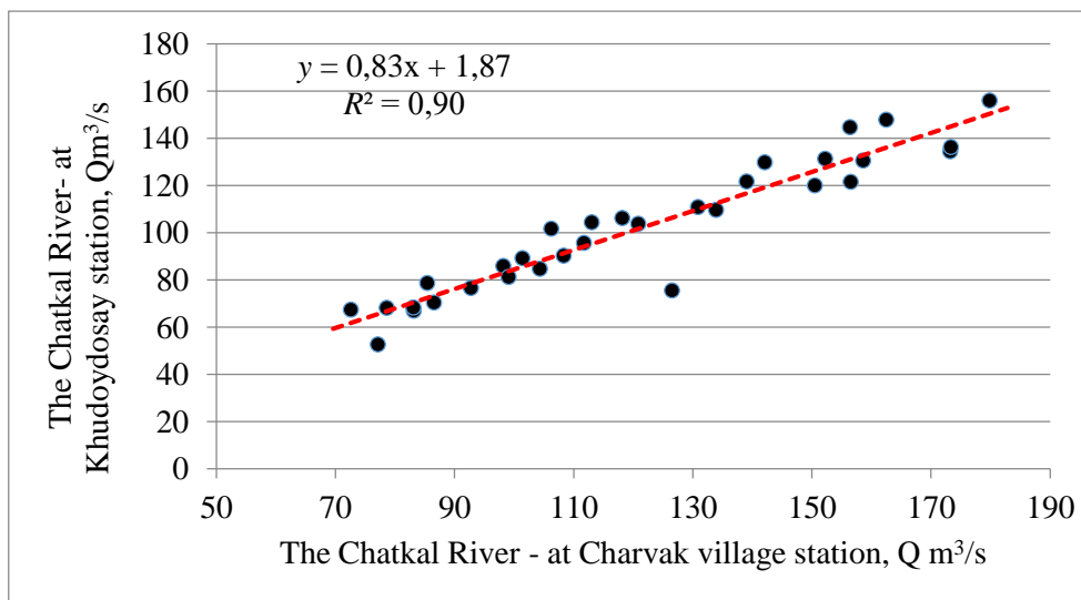
Fig. 1. Average-flow correlations between two The Chatkal River streams, Khudoydodsay station and Charvak village station, 1933-1966.
