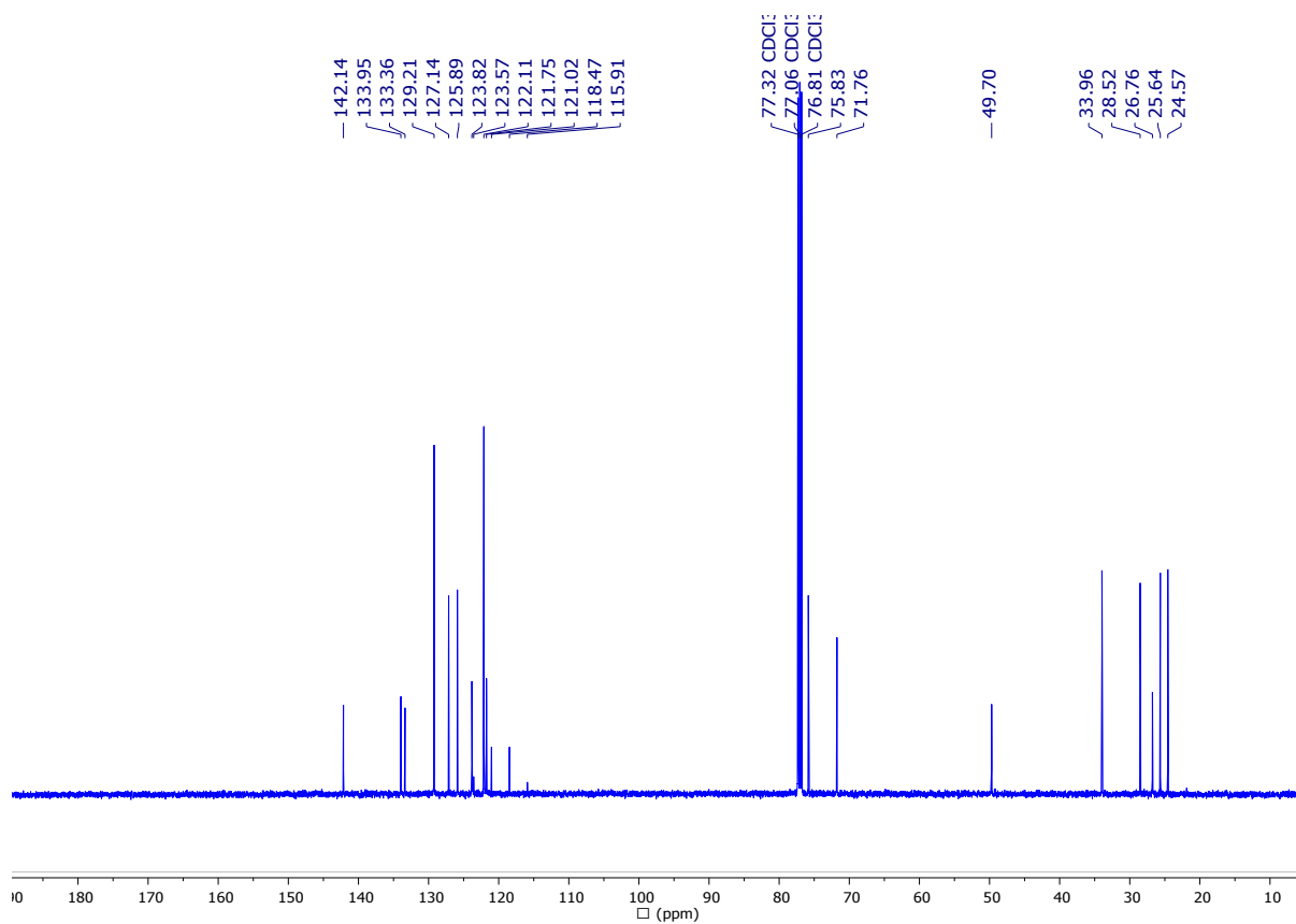
Figure S10 – ^{13}\text{C} NMR spectrum of compound 6 (400 MHz, \text{CDCl}_3 , 25 ^\circ\text{C} ).
