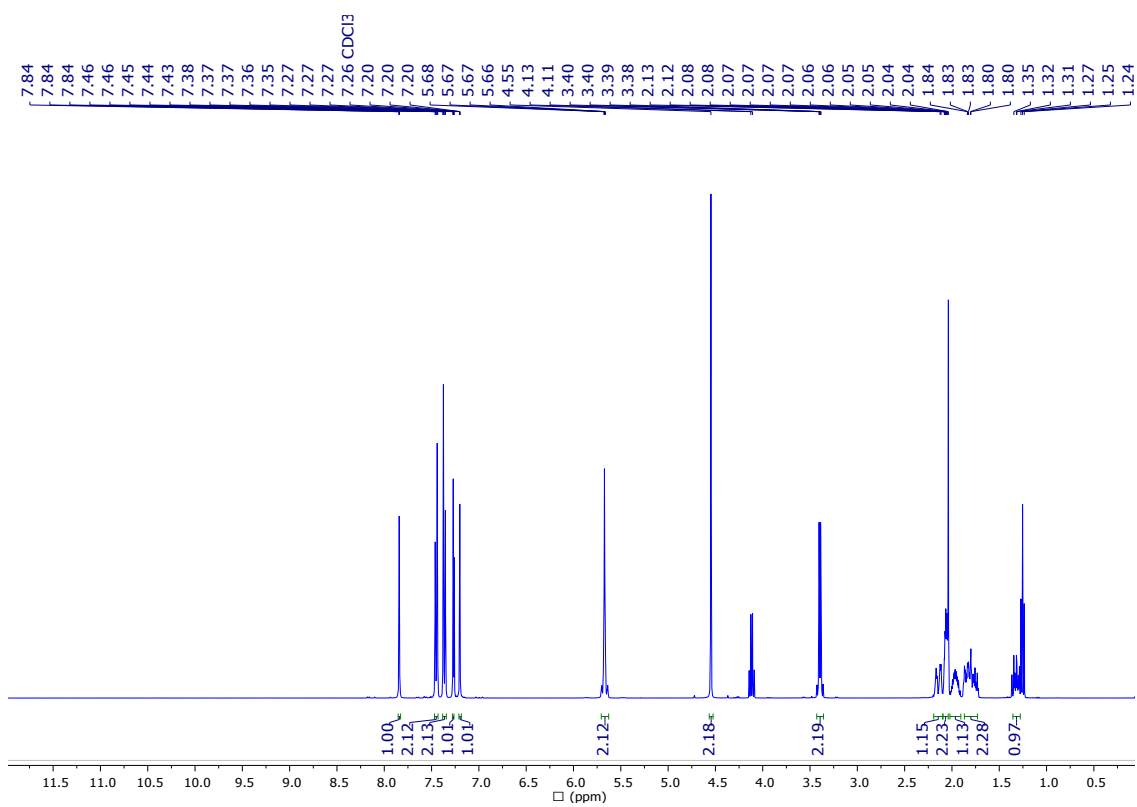
Figure S5 – ^1\text{H} NMR spectrum of compound 4 (400 MHz, \text{CDCl}_3 , 25 °C).
