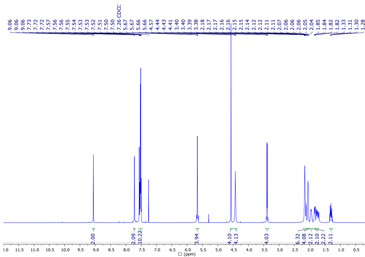
Figure S9 – ^1\text{H} NMR spectrum of compound 6 (400 MHz, \text{CDCl}_3 , 25 ^\circ\text{C} ).
