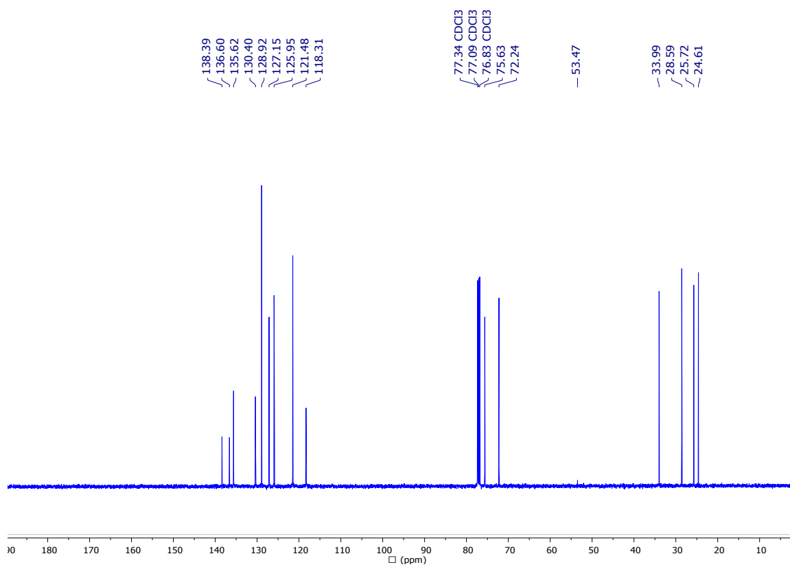
Figure S6 – ^{13}\text{C} NMR spectrum of compound 4 (400 MHz, \text{CDCl}_3 , 25 °C).
