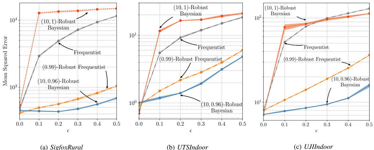
Fig. 7: Test mean squared error (33) as a function of the corruption level \epsilon of the standard frequentist solution based on the log-loss, the robust frequentist solution based on the t -log-loss with t = 0.99 , and the (m, t) -robust Bayesian learning with m = 10 and t = \{1, 0.96\} . As \epsilon increases, the training data sets are increasingly affected by outliers.
