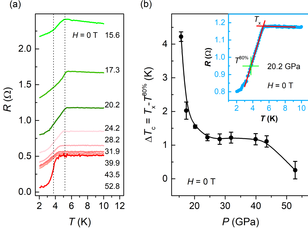
FIG. 4. (a) The SC transition of \text{Rb}_2\text{Mo}_6\text{Se}_6 at different pressure and zero field ( H = 0 T). Dashed lines are guides to the eye. (b) Zero-field superconducting transition widths as a function of pressure. The insert exemplifies the method of determining \Delta T_c = T_x - T^{80\%} . We derive T^{80\%} = (0.8bT_x + 0.8a - a')/b' from the same coefficients a , b , a' , and b' as explained above and calculate \Delta T_c = T_x - T^{80\%} .
