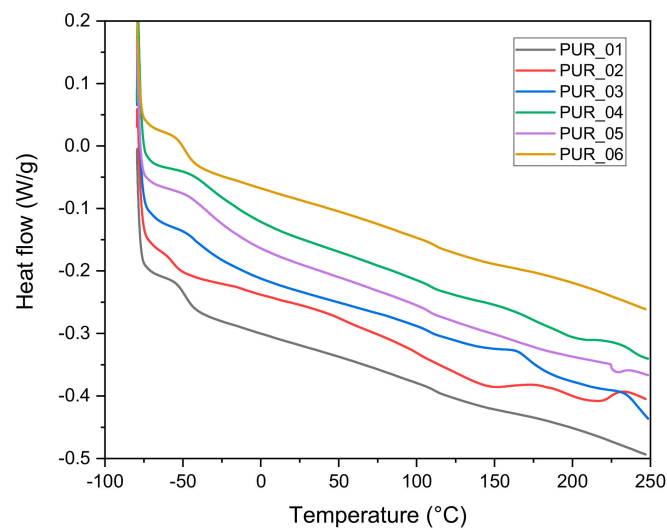
Figure 9. DSC thermograms of polyurethane foams ( 10 \text{ K} \cdot \text{min}^{-1} ).
