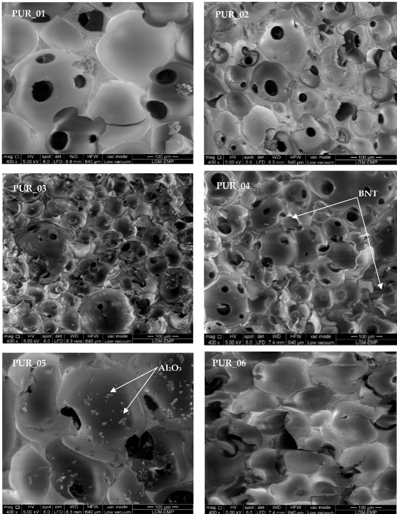
Figure 12. SEM micrographs showing the PUR pores and distribution of BNT and Al 2 O 3 particles.
