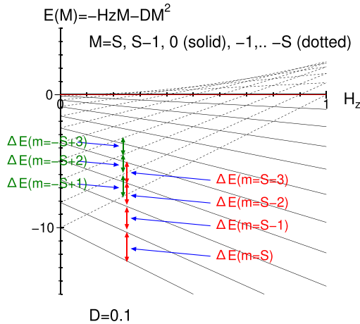
FIG. 2. Energy levels of the spin S = 10 as a function of positive H_z for D = 0.1 . Some of the energy differences between the states are depicted by arrows.
