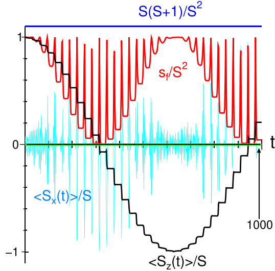
FIG. 6. Motions of spin S = 10 for H_z = 0.1 , h_{ac} = 0.005 , and the driving ac field f(t) given by Eq. (8). The amplitude h_{ac} = 0.005 . \langle S_x(t) \rangle (thin curve) and \langle S_z(t) \rangle (bold curve) are normalized by S . The normalized spin length (spin fidelity s_f ) is given by the bold line (above). The total spin S(S+1) normalized by S^2 is given by the blue line.
