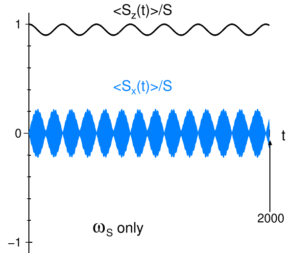
FIG. 3. Time dependence of the reduced spin components S_x(t)/S (below, thin line) and S_z(t)/S (above, bold line) under the ac field of \omega_{S \rightarrow S-1} only. h_{\text{ac}} = 0.005 . (In the figure \omega_S denotes \omega_{S \rightarrow S-1} .) The initial state is (S_x/S, S_y/S, S_z/S) = (0, 0, 1) . As we have S = 10 , this scheme shows that S_x oscillates between +2 and -2 and S_z between S = 10 and S - 1 = 9 .
