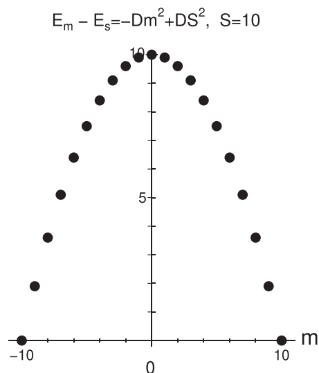
FIG. 1. Energies of states E_m [Eq. (2)] for S = 10 , D = 0.1 , and H_z = 0 . We plot E_m - E_{\min} , E_{\min} = E(\pm S) = -DS^2 , showing the energy barrier between the states m > 0 and m < 0 .
