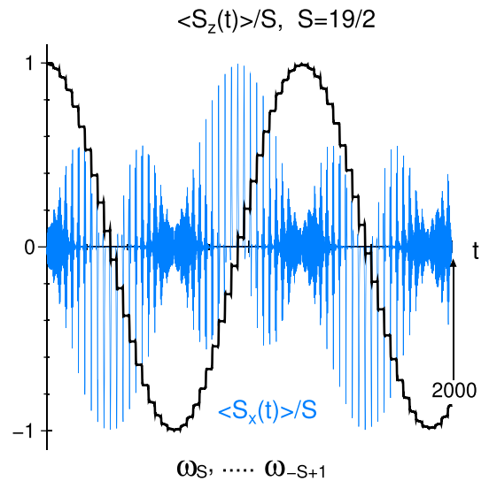
FIG. 5. Time dependence of the reduced spin components S_x(t)/S (below, thin line) and S_z(t)/S (above, bold line) under the ac field of \omega_{S \rightarrow S-1}, \dots, \omega_{-S+1 \rightarrow S} for a noninteger spin S = 19/2 . H_z = 0 and h_{ac} = 0.005 . (In the figure \omega_S represents \omega_{S \rightarrow S-1} , and so on.) The initial state is (S_x, S_y, S_z) = (0, 0, 1) .
