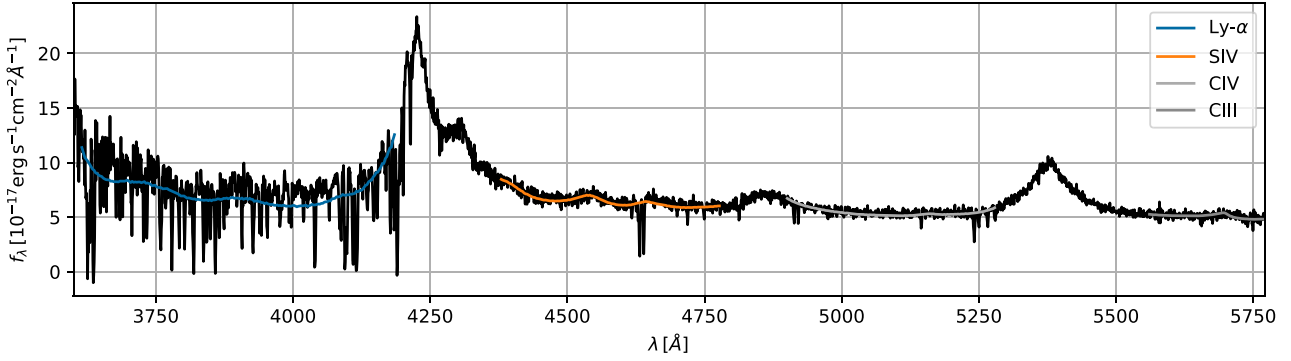
Figure 9. Example of a high signal-to-noise quasar spectrum. The mean expected flux \bar{C}(\lambda_{\text{RF}}) as in equation (4) is shown for the Lyman- \alpha , S IV, C IV, and C III regions. The quasar has a redshift z_q = 2.495 and is identified as a DESI object with TARGETID = 39628443918272474. As in this example, we occasionally observe metal absorption in the calibration regions.
