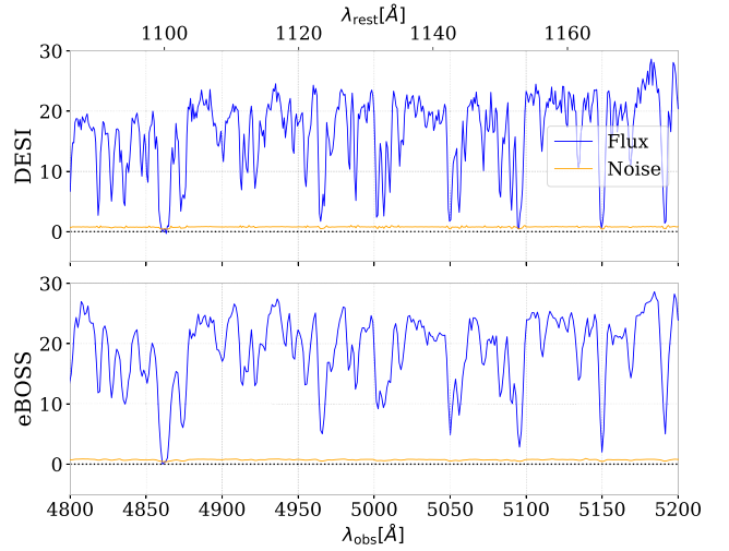
Figure 4. Illustration of the resolution improvement between eBOSS and DESI. The DESI spectrum of the quasar represented in Fig. 1 is zoomed on a region of the Ly \alpha forest on the top panel. The spectrum of the same quasar obtained by the SDSS-IV (Gunn et al. 2006; Smee et al. 2013; Dawson et al. 2016; Blanton et al. 2017) in the 16th Data Release (DR16; Ahumada et al. 2020) of the eBOSS. The SDSS name associated with this quasar is 142 903.03–014 519.3. The DESI spectrum is obtained after three individual exposures for a total exposure time of 2300 s. The eBOSS spectrum have 11 exposures for a total of 6300 s. The large-scale absorption structures are similar but due to its improved spectroscopic resolution, the DESI spectrum clearly shows more details at small scales.
